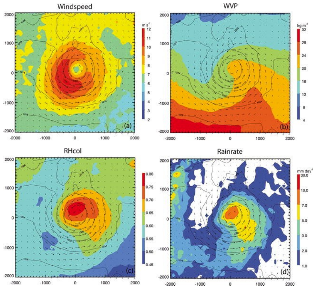
Fig. 1 North Atlantic composite mean fields from \sim 400 individual cyclones. The mean field mean sea level pressure and surface wind vectors are overplotted in each diagram. The filled contours represent (a) surface wind speed, (b) water vapor path, (c) column relative humidity and (d) rain rate (from Field and Wood, 2007).
