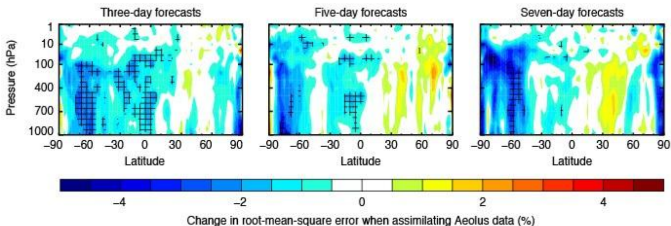
Figure 1: Change in wind forecast errors (shading) through the assimilation of Aeolus data during 2 August–18 October 2019. Cross-hatching indicates statistical significance at the 5% level. Credit: ECMWF.
