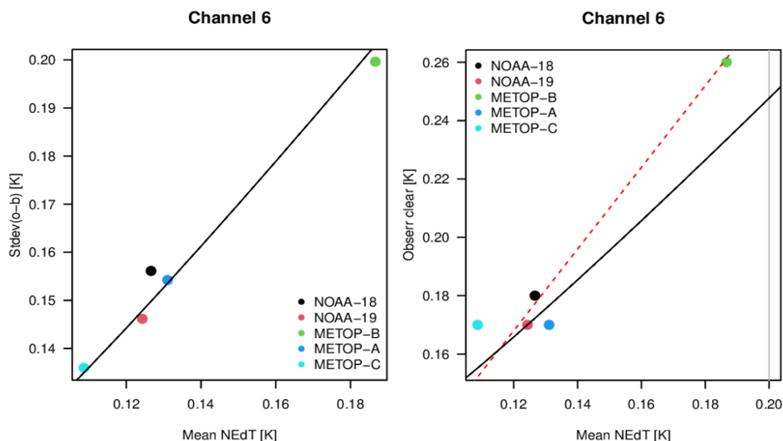
Figure 17: Standard deviation of O-B vs. sample NEDT (left) and assigned clear sky observation errors vs. sample NEDT (right) for AMSU-A channel 6 on various satellite platforms. Fitted lines show the results from using a simple scaling of sample NEDT (red dashed) or using equation 7 (solid black line). The grey line indicates the sample noise for the small satellite after 3x3 averaging. Data are from 13-31 May 2021.
