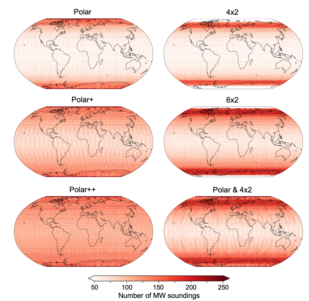
Figure 4: Maps showing the density of all simulated MW observation locations after thinning accumulated over two days (8-9 Jun 2018) for the six potential small satellite constellations tested (table 2).
