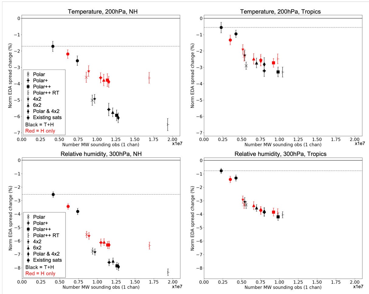
Figure 7: As for figure 6 but for temperature at 200hPa (top row) and humidity at 300hPa (bottom row) in the northern hemisphere (latitude > 20^{\circ}\text{N} ) (left panel) and tropics ( 20^{\circ}\text{S} < \text{latitude} < 20^{\circ}\text{N} ) (right panel).
