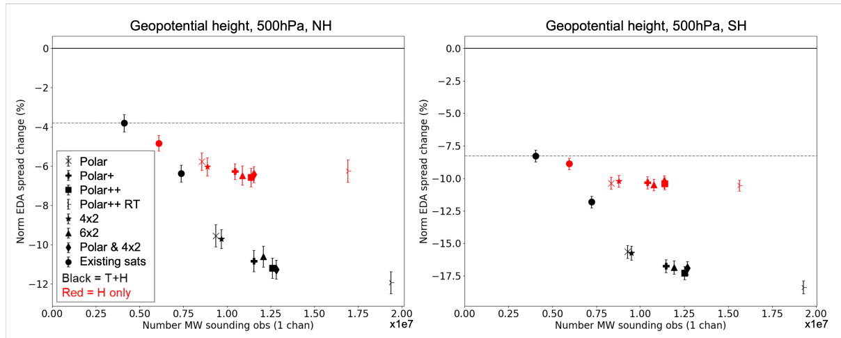
Figure 6: Percentage EDA spread reductions with increasing observation numbers for geopotential height at 500hPa from a baseline with no MW sounder data for all constellation options and baselines. Black and red symbols indicate respectively the addition of temperature and humidity sounding channels or humidity channels only to the Metop/JPSS baseline. Different symbols denote the different simulated data scenarios or the use of real MW data where the additional “Polar++ RT” refers to a reduced thinning sensitivity experiment (see section 5.2). The point furthest left, picked out on the dotted grey line, corresponds to the Metop/JPSS baseline to which all other combinations of real and simulated data are added. Data are from the northern hemisphere (latitude > 20^{\circ}\text{N} , left panel) and southern hemisphere (latitude > 20^{\circ}\text{S} , right panel) over the period 8-28 June 2018. Error bars indicate an estimate of 95% confidence.
