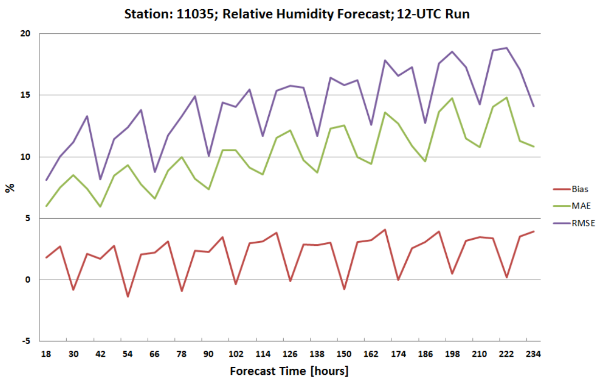
Figures 5-8 Mean error (bias), mean absolute error (MAE) and RMSE of ECMWF point forecasts of 10m wind speed and direction, 2m temperature and 2m relative humidity as a function of forecast range for station VIENNA in the period Jan-Dec 2014.
