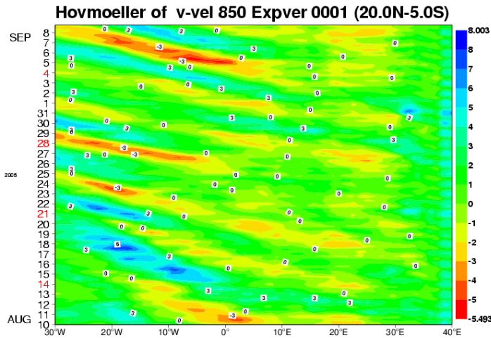
Figure 1.11: Hovmöller longitude-time plot of 6-hourly analysed ECMWF 850 hPa v velocities averaged over 5S-20N between 10 August and 9 September 2005.
