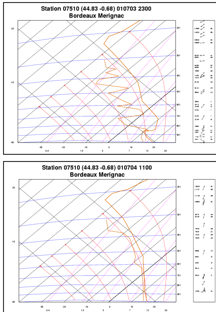
Figure 4.7: Tephigrams of observed soundings at Bordeaux-Merignac (France) for 4 July 2001 00 UTC (top), and 12 UTC (bottom).
