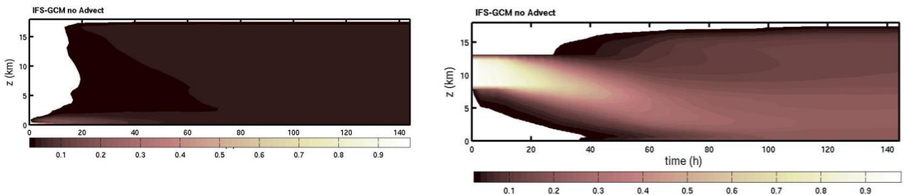
Figure 3.9: Same as Figure 3.8 but from a global IFS simulation at resolution T159 initialized with ERA40. For better comparison, the horizontal advection has been switched off for tracers.
