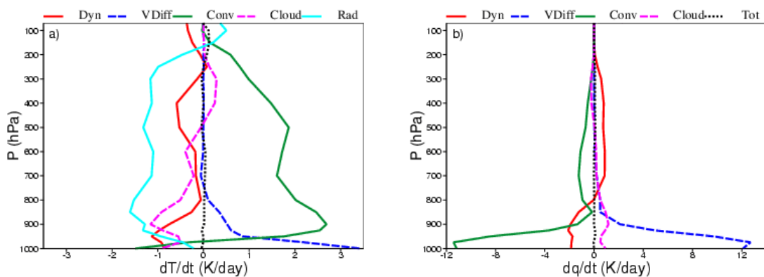
Figure 1.3: Tendencies from the different physical processes as computed in the IFS and averaged over the tropical belt between 20\text{N}\text{--}20\text{S} . Dyn denotes the dynamical tendency (horizontal + vertical advection), VDiff the contribution from the boundary-layer diffusion scheme, Conv the contribution from shallow and deep convection, Cloud the large-scale condensation/evaporation processes, and Rad the radiation.
