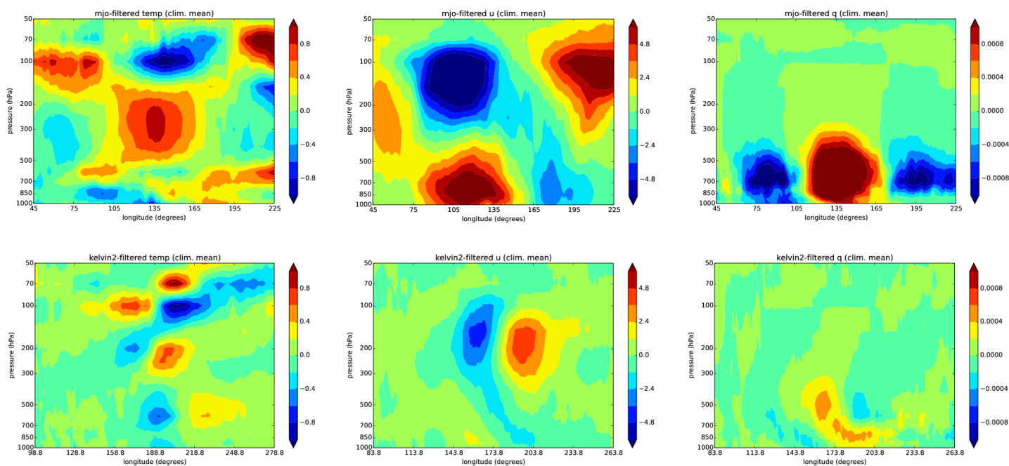
Figure 5.4: Composite of - from left to right - T (K), u ( \text{m s}^{-1} ) and q ( \text{g kg}^{-1} ) anomalies for the MJO mode, top row, and the Kelvin wave mode, bottom row, from the ECMWF operational analysis. The composites are obtained by regression of the time series onto the point with maximum OLR variance in either the MJO or Kelvin spectral bands –courtesy Michael Hermann for the wave analysis package.
