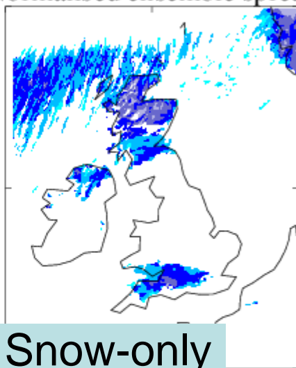
Normalised ensemble spread
