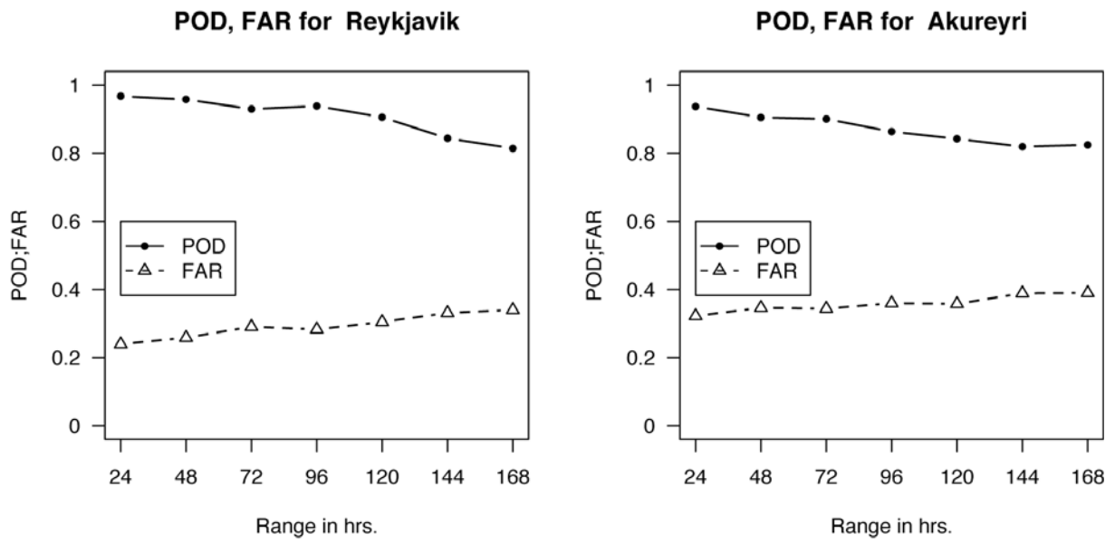
Fig.4 Probability of detection (POD) and False Alarm Rate (FAR) for left: Reykjavík (WMO 4030) and right: Akureyri (WMO 4063) in 2008.
