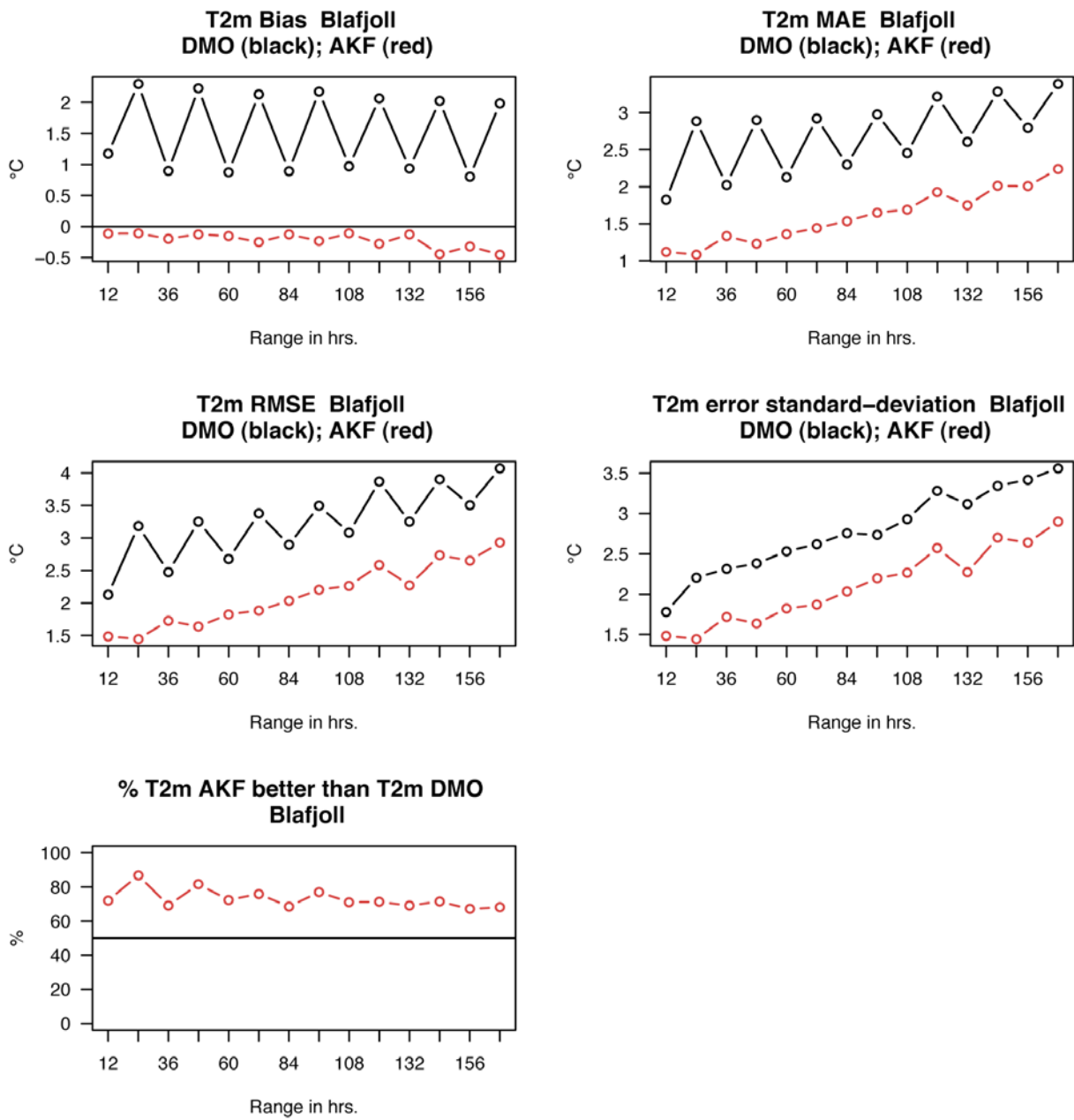
Fig.2 Verification of ECMWF (12 UTC run) DMO and Kalman filtered 2-metre temperature forecasts for Bláfjöll (WMO 4138) in 2008. Statistical scores versus forecast range.
