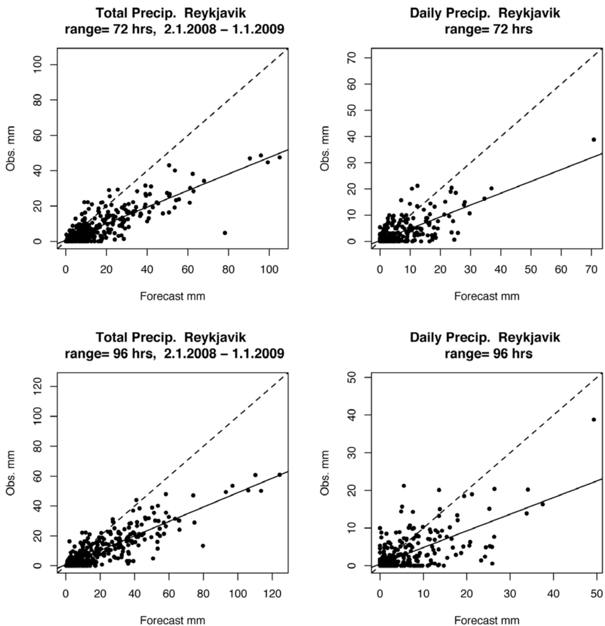
Fig.3 Verification of ECMWF precipitation forecasts (12 UTC run) for Reykjavík (WMO 4030) in 2008. Top left: accumulated precipitation in 72h valid at T+72h, top right: 24h accumulated precipitation valid at T+72h. Bottom left: accumulated precipitation in 96h valid at T+96h and bottom right: 24h accumulated precipitation valid at T+96h.
