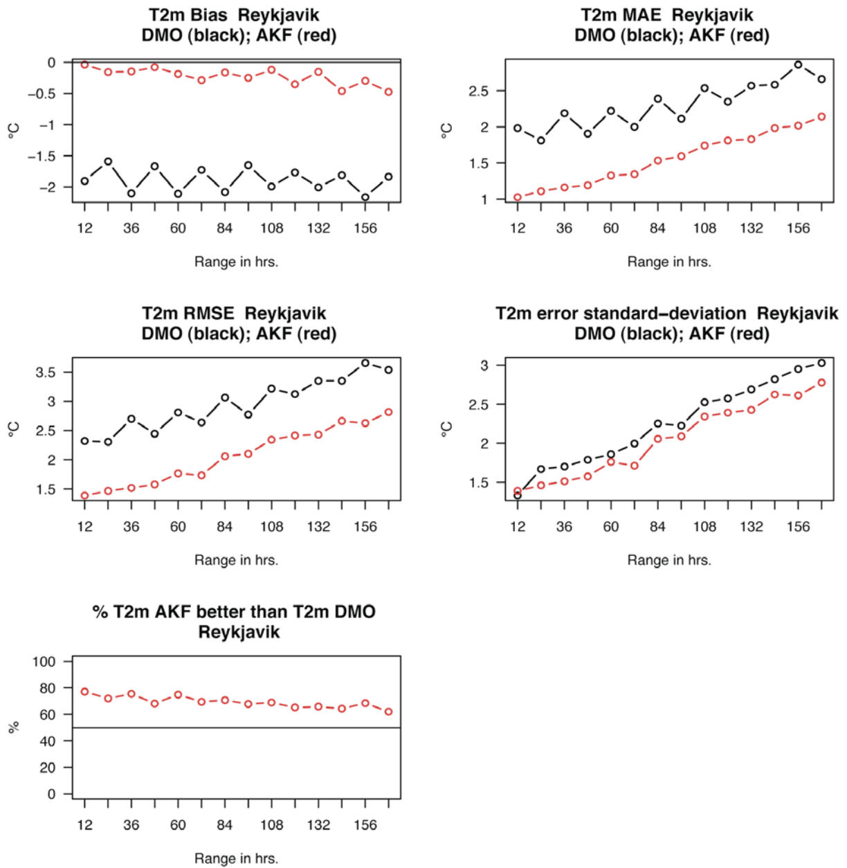
Fig.1 Verification of ECMWF (12 UTC run) DMO and Kalman filtered 2-metre temperature forecasts for Reykjavik (WMO 4030) in 2008. Statistical scores versus forecast range.
