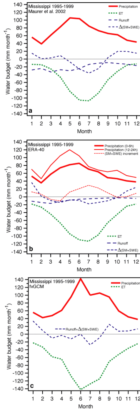
Figure 2 Water budget annual cycle for the Mississippi basin from Maurer et al. [2002], ERA-40, and fvGCM for 1995-1999.
