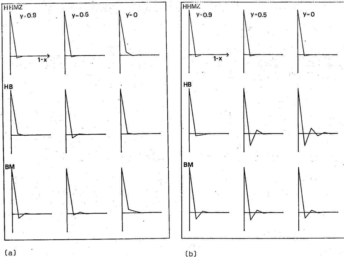
Fig. 4 - Boundary layers for modified test problem and each method (a) for mesh Péclet number \beta = 20 and (b) for \beta = 100 .
