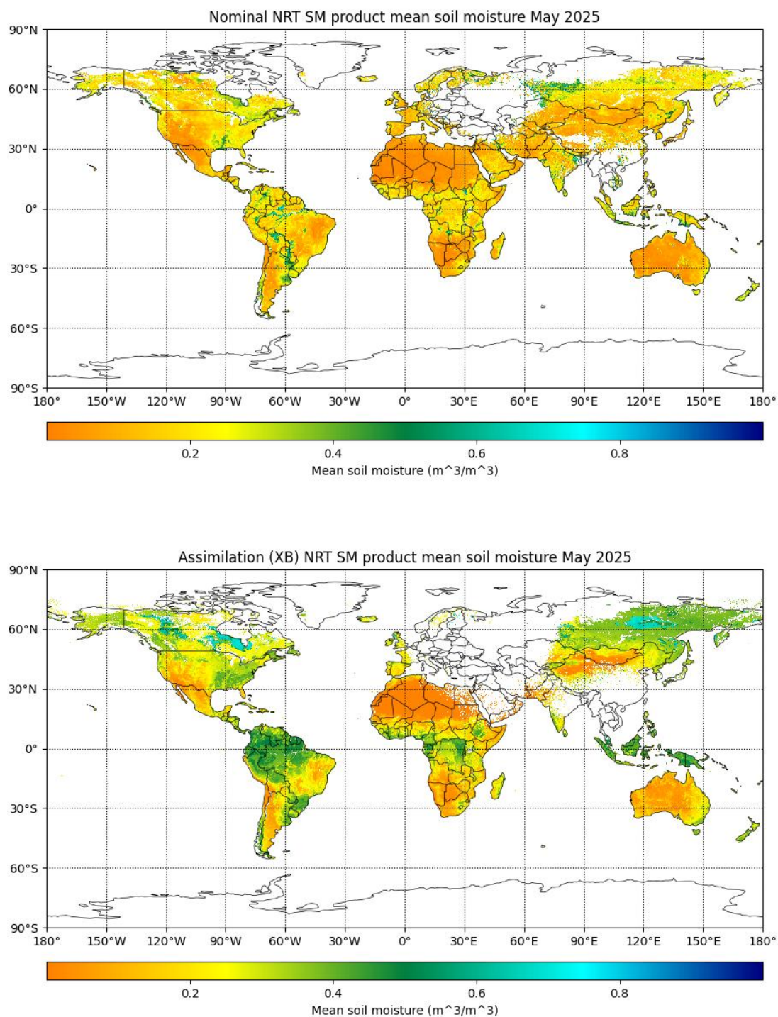
Figure 3: Mean retrieved soil moisture ( \text{m}^3/\text{m}^3 ) for May 2025 for the nominal NRT product (upper) and assimilation NRT product (lower)
