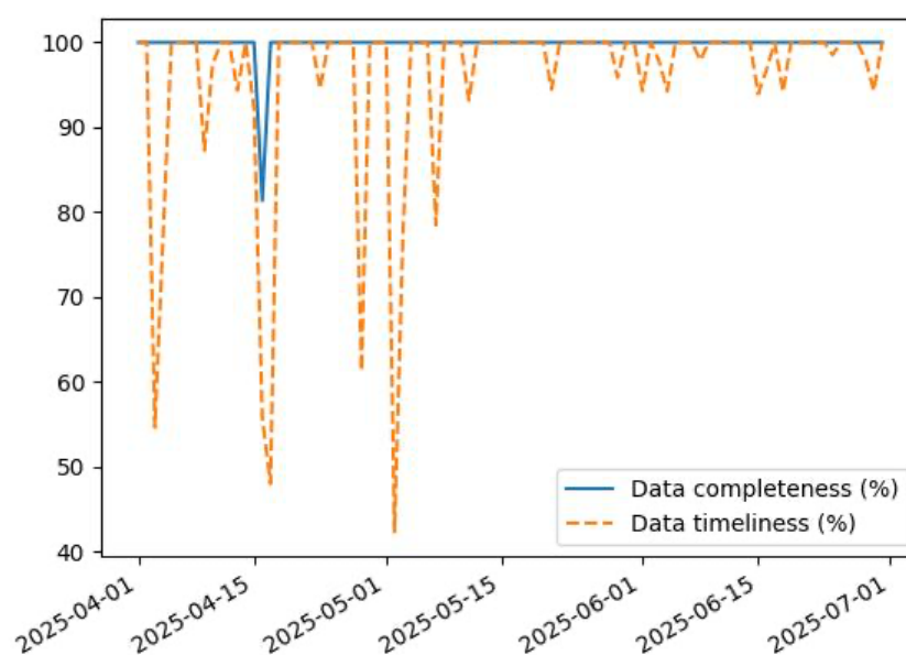
Figure 1: Daily SMOS NN nominal soil moisture production completeness and delivery timeliness percentages (see text for how these are calculated) for the second quarter of 2025: 1 st April to 30 th June 2025
