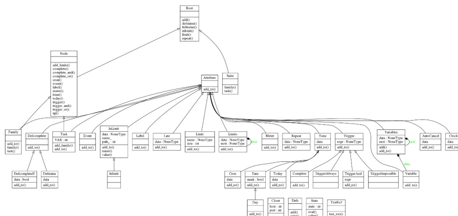
Figure 3.1 Class Diagram for module ecf.py .
