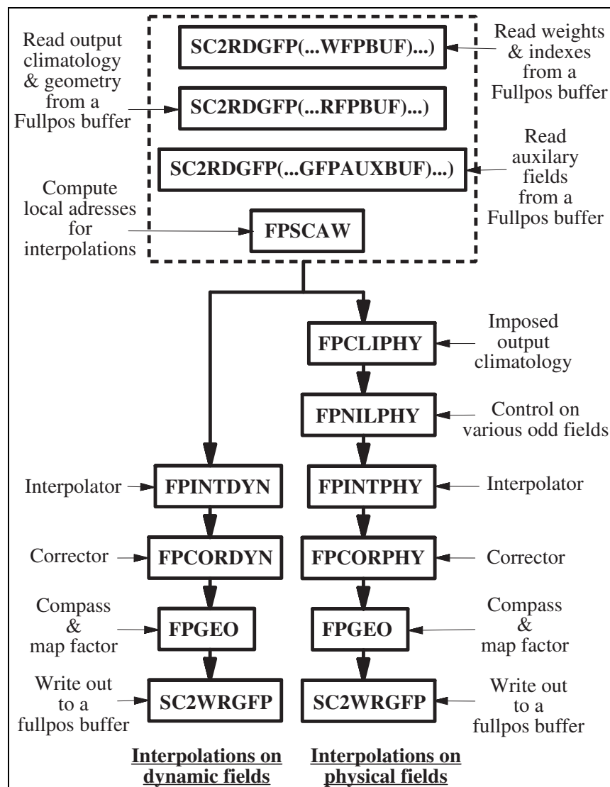
Figure 2.12 Horizontal interpolations management: FPOSHOR.
