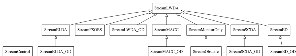
Class Diagram for module inc_stream.py .
