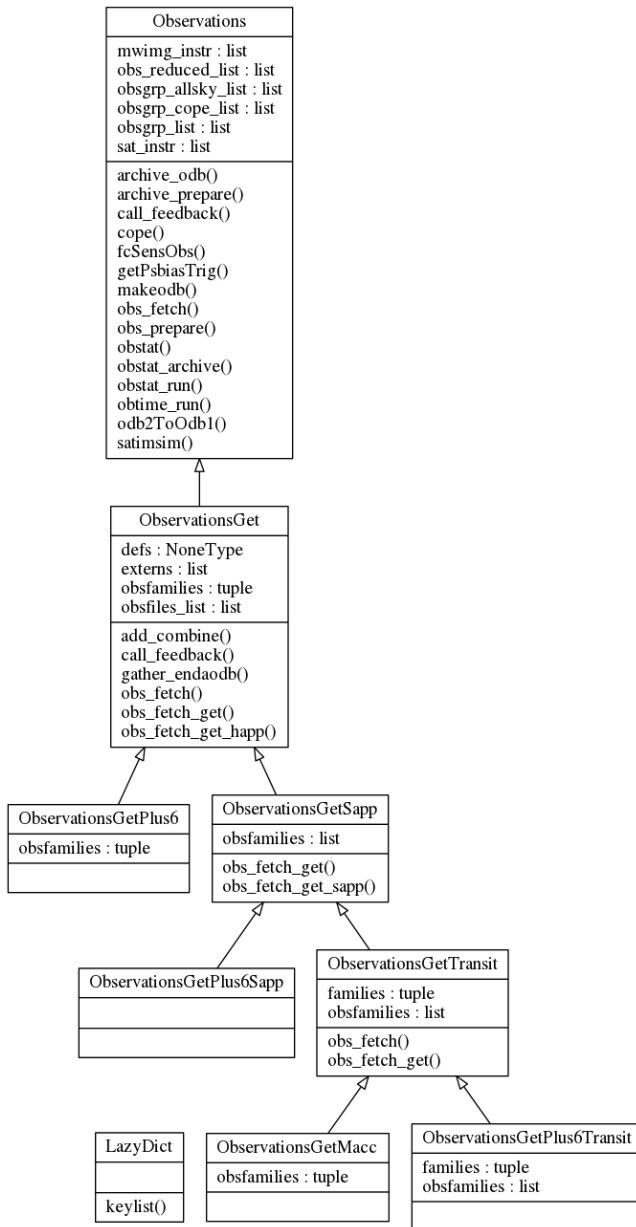
Class Diagram for module inc_obs.py.
