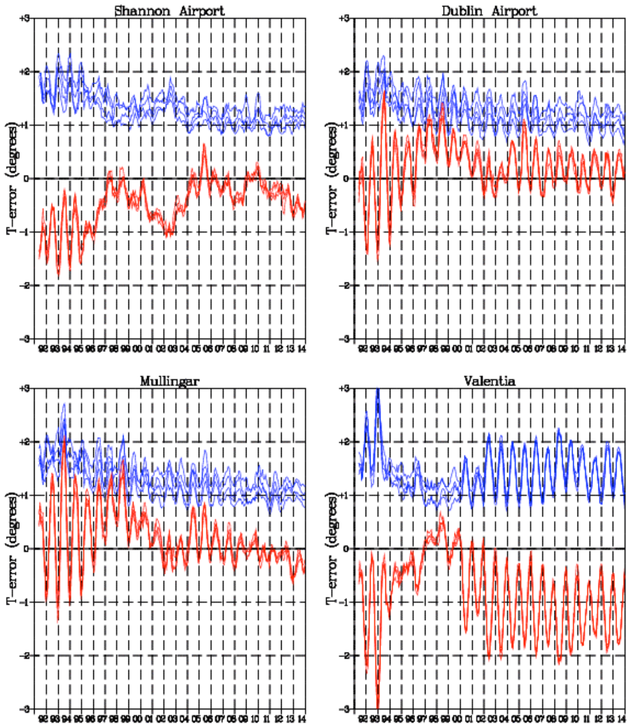
Smoothed Monthly Scores [Mean/Abs] for Temperature Forecasts Verifying at Midday
