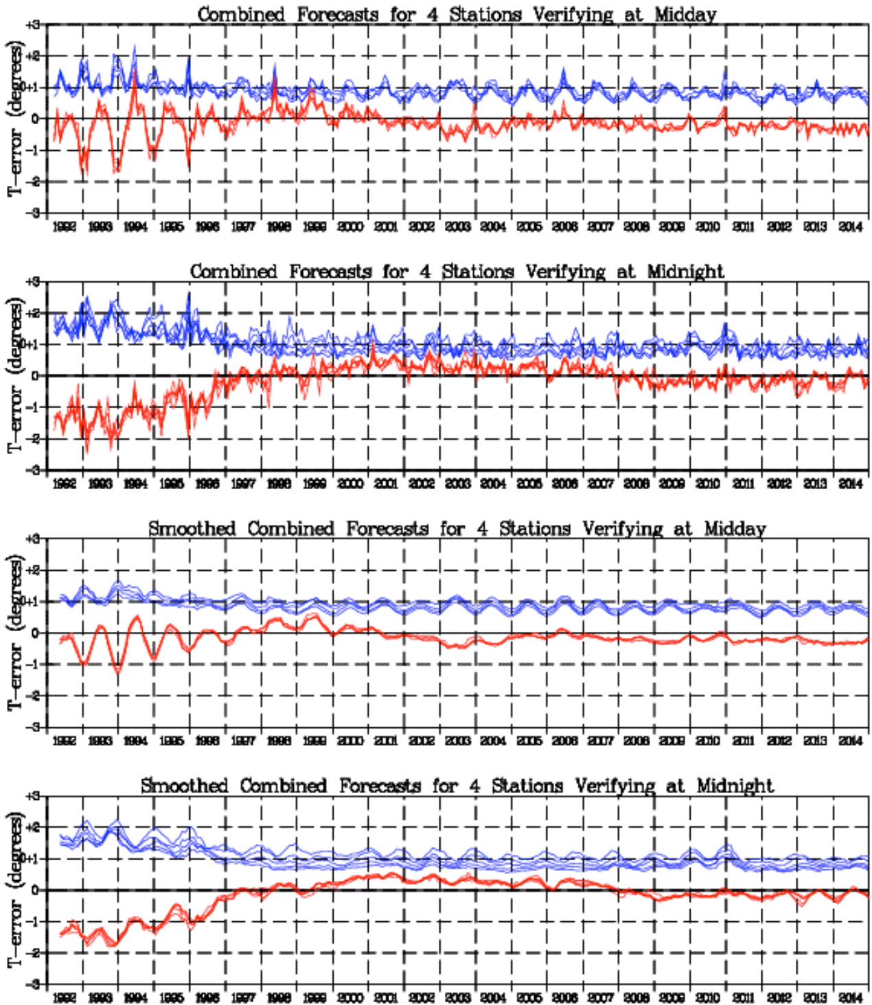
Fig. 5 Mean monthly scores for ECMWF forecasts of 2-metre Temperature averaged over four stations. The top two graphs show the scores for midday [T+24, T+48, T+72, and T+96] and midnight [T+12, T+36, T+60, T+84, and T+108], respectively, without smoothing; the bottom two graphs show the effects of smoothing. The blue lines indicate the error [mean absolute error], the red lines the bias [mean error]. In all cases the top blue line corresponds to the longest forecast, the bottom blue line to the shortest.
