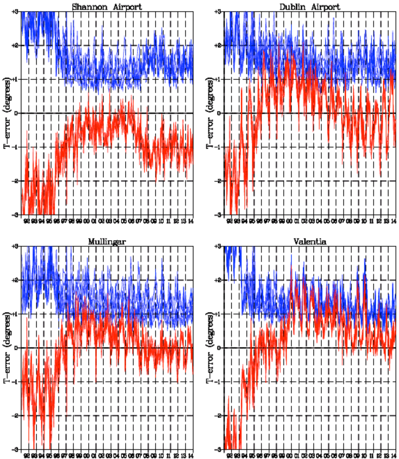
Fig 2 Scores for the T+12, T+36, T+60, T+84, and T+108 ECMWF forecasts of 2-metre Temperature. Note that all these forecasts verify at midnight. The blue lines show values of the monthly mean of the absolute error, the red lines values of the monthly mean of the mean error or bias.
