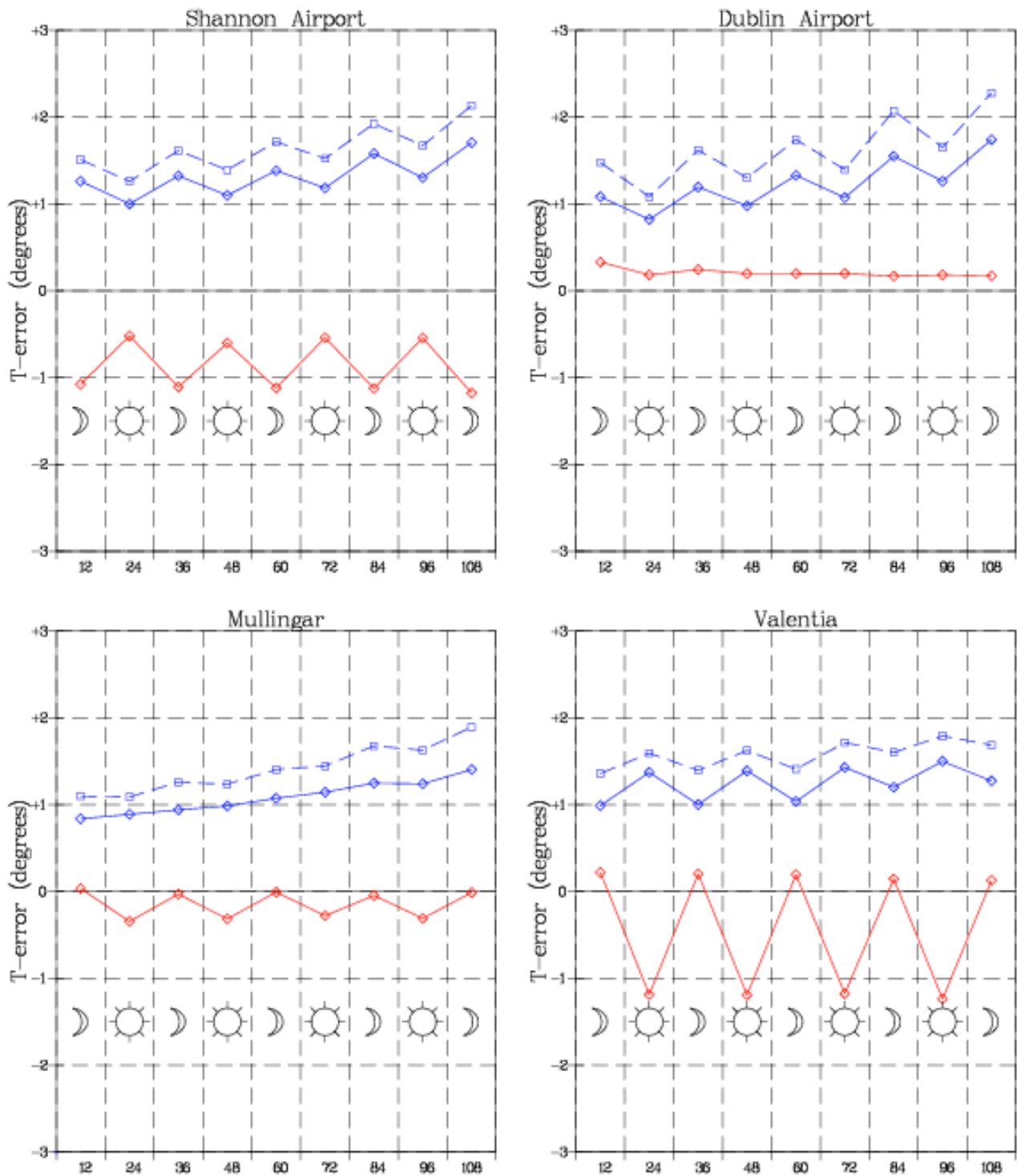
Scores [Mean/Abs/RMS] for Temperature Fcsts Verifying Midday and Midnight in 2014
