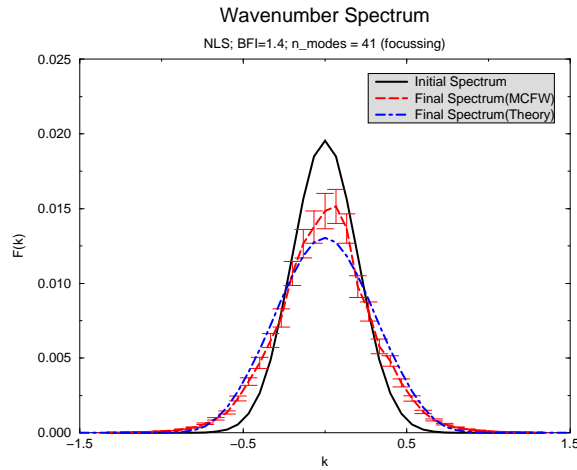
Figure 4: Initial and final time wave number spectrum according to the Monte Carlo Forecasting of Waves (MCFW) using the nonlinear Schrödinger Equation. Error bars give 95% confidence limits. Results from theory are shown as well.
