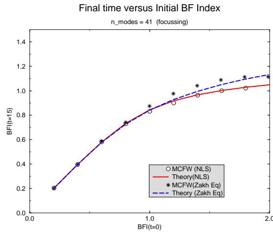
Figure 11: Comparison of curves of final time versus initial value of the BF Index from simulations with the nonlinear Schrödinger equation and from the Zakharov equation. The corresponding theoretical results are shown as well.
