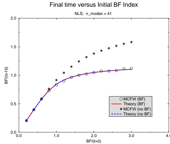
Figure 6: Final time versus initial time value of the BF Index for the same cases as displayed in Fig. 5.
