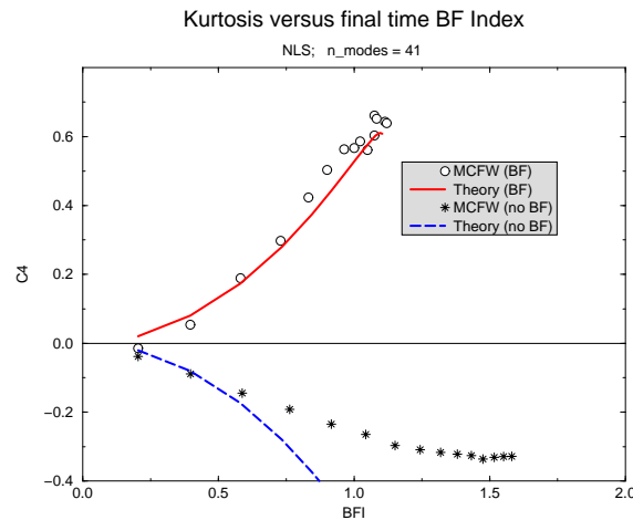
Figure 8: Normalized Kurtosis as function of the BF Index. Shown are results for focussing (BF) and defocussing (no BF) from the simulations and from theory. The theoretical result for defocussing can be obtained from the results of focussing by a reflection with respect to the x -axis.
