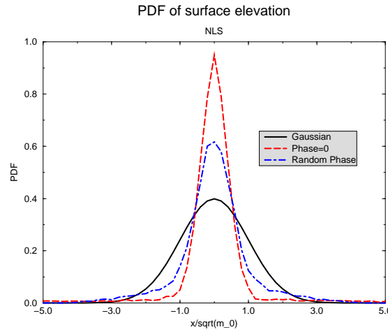
Figure 2: The surface elevation probability distribution as function of normalized height, \eta/\sqrt{m_0} (with m_0 the variance), corresponding to the cases of Fig. 1. For reference the Gaussian distribution is shown as well.
