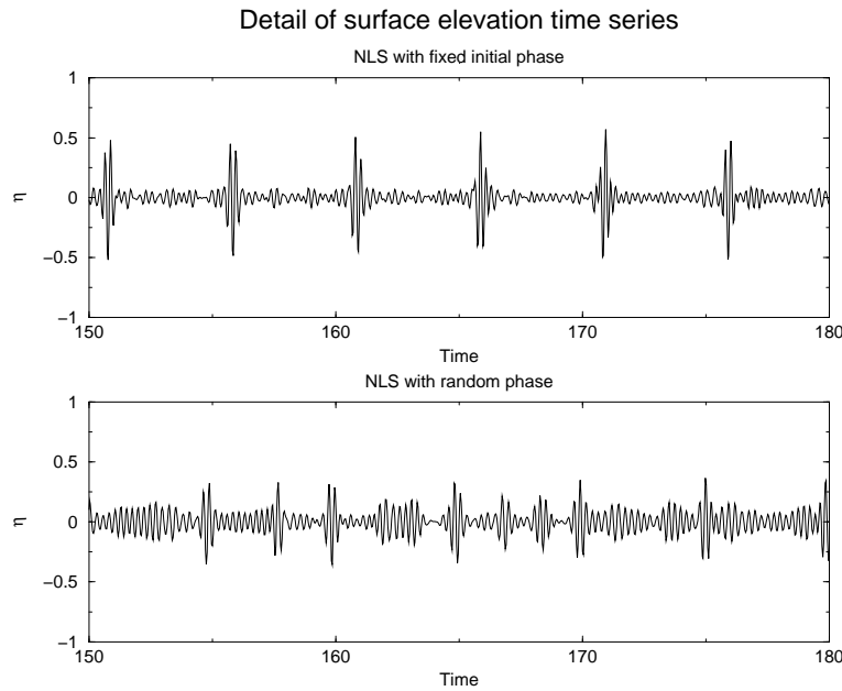
Figure 1: Detail of surface elevation \eta as function of dimensionless time t' . The top panel a) shows the time series for a fixed choice of initial phase, \theta = 0 , while the bottom panel b) shows the time series for a random choice of initial phase.
