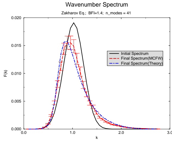
Figure 10: Initial and final time wave number spectrum according to Monte Carlo Forecasting of Waves (MCFW) using the Zakharov equation. Error bars give 95% confidence limits. Results from theory are shown as well.
