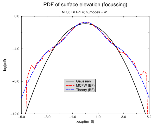
Figure 7: Probability distribution function for surface elevation as function of normalized height \eta/\sqrt{m_0} . Results from numerical simulations with the nonlinear Schrödinger equation and homogeneous theory in case of focussing (BF Index of 1.4). For reference the Gaussian distribution is shown as well. Freak waves correspond to a normalized height of 4.4 or larger.
