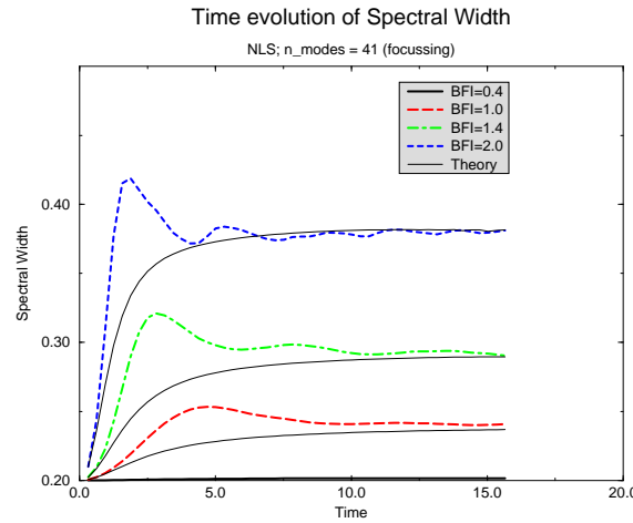
Figure 3: Time evolution of spectral width for several values of the BF Index. Corresponding results from homogeneous theory are shown as well.
