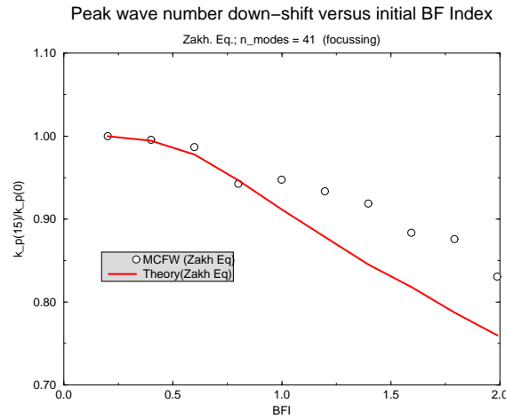
Figure 13: Final time peak wave number down-shift versus BF Index. Shown is a comparison between numerical simulation results from the Zakharov equation and theory.
