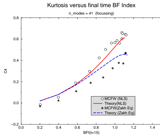
Figure 12: Normalized Kurtosis as function of the BF Index. Shown are results for focussing from simulations with the nonlinear Schrödinger equation and with the Zakharov equation. The corresponding theoretical results are shown as well.
