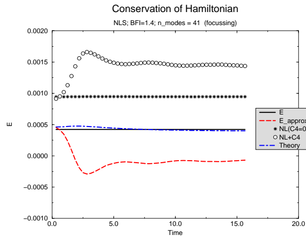
Figure 15: Time evolution of Hamiltonian E of the nonlinear Schrödinger equation. Also shown are time evolution of E according to lowest order inhomogeneous theory ( E_{approx} ) and according to homogeneous theory that includes the fourth cumulant. Finally, shown are the nonlinear contribution to E for a strictly Gaussian state ( NL(C4=0) ), and including all higher order cumulants ( NL+C4 ).
