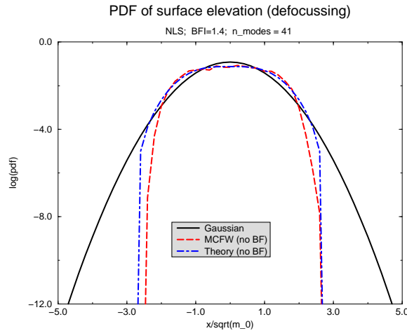
Figure 9: Probability distribution function for surface elevation as function of normalized height \eta/\sqrt{m_0} . Results from numerical simulations with the nonlinear Schrödinger equation and homogeneous theory in case of defocussing (BF Index of 1.4). For reference the Gaussian distribution is shown as well.
