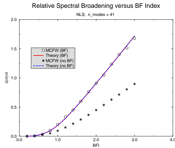
Figure 5: Relative spectral broadening (\sigma_k(t_\infty^l) - \sigma_k(0))/\sigma_k(0) as function of the BF Index. Shown are results for focussing (BF) and defocussing (no BF) from the simulations and from theory, but results from theory are identical for these two cases.
