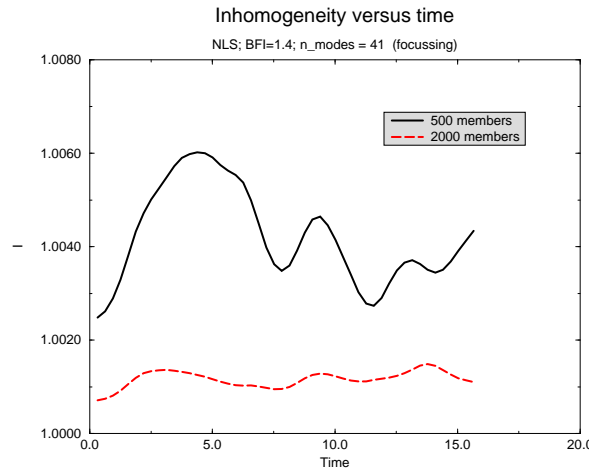
Figure 14: Time evolution of a measure for inhomogeneity, I , for two different ensemble sizes, according to the nonlinear Schrödinger equation.
