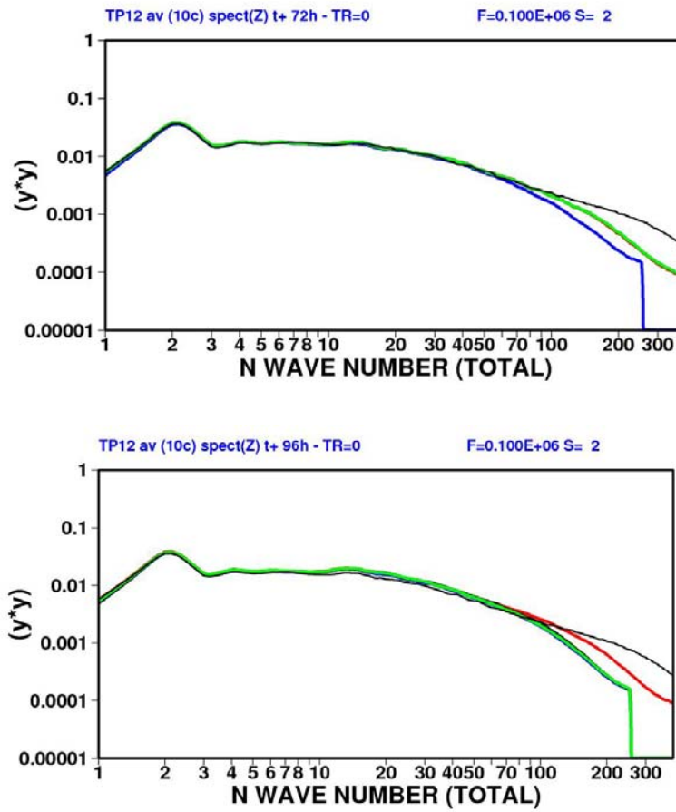
Figure 5 Spectra of the squared ensemble forecasts of 12-hour accumulated total precipitation ( TP12^2 ) for the T399 (red solid lines), T255 (blue solid lines), VAR3-OV-24HD (black solid lines) and VAR3 (green solid lines) ensembles at t+72h (top panel) and at t+96h (bottom panel). The thin black solid line visible in both panels shows the spectra of a proxy of verification given by the t+12h and the t+24h TP12 forecast by the operational, T799 ECMWF forecast. At t+72h , the T399 and VAR3-OV-24HD curves coincide with the VAR3 line and thus are not visible, while at t+96h the VAR3-OV-24HD and VAR3 curves are very similar to the T255 curve. TP12^2 values (in m^2 ) have been multiplied by 10^{-5} .
