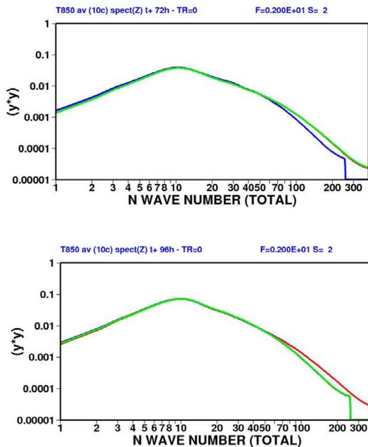
Figure 8. As Fig. 7 but for the spectra of the ensemble variance of the 850 temperature (T850) for the T399 (red solid lines), T255 (blue solid lines), VAR3-OV-24HD (black solid lines) and VAR3 (green solid lines) ensembles at t+72h (top panel) and at t+96h (bottom panel). At t+72h, the T399 and VAR3-OV-24HD curves coincide with the VAR3 line and thus are not visible, while at t+96h the VAR3-OV-24HD and VAR3 curves are very similar to the T255 curve. STD^2 values (in degrees) have been multiplied by 0.5.
