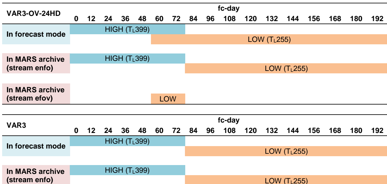
Figure 1. Schematic of the VAR3-OV-24HD and the VAR3 configurations. The VAR3-OV-24HD EPS uses a 24h overlap period: the low-resolution ( T_{L255} ) forecast starts at t+48h and have a 24h overlap with the high-resolution ( T_{L399} ) forecast. The ensemble archive (stream enfo) contains the high-resolution fields between 0 and t+72h , and the low-resolution fields from t+72h . The low-resolution fields produced between t+48h and t+72h can be accessed from the archive stream efov. The VAR3 EPS does not have any overlap period: the low-resolution ( T_{L255} ) forecast starts at t+72h .
