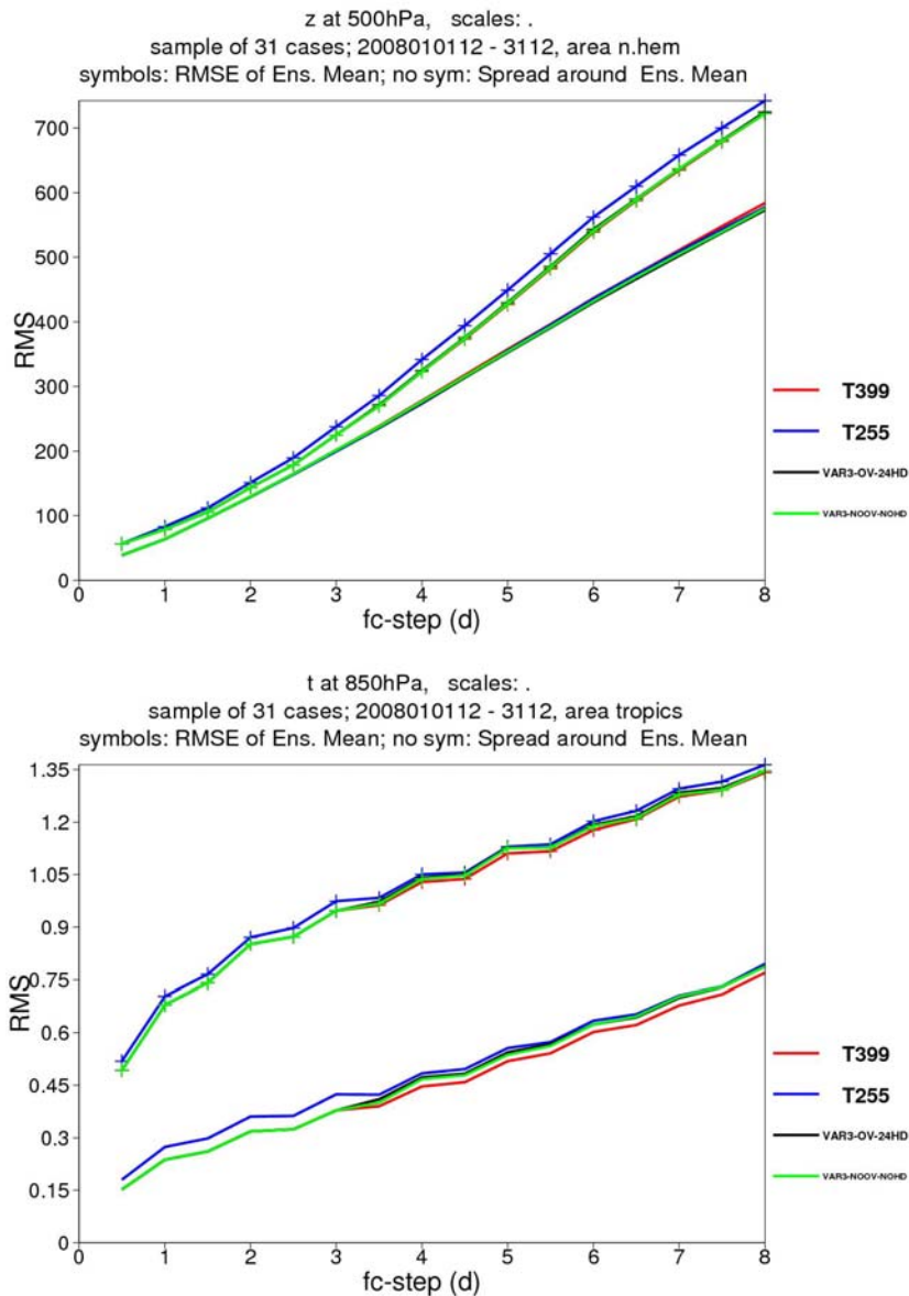
Figure 2 Root-mean-square-error (RMSE) of the ensemble-mean forecast (solid lines with symbols) and ensemble standard deviation (solid lines) of the T399 (red), T255 (blue), VAR3-OV-24HD (black) and VAR3 (green) ensembles, computed for Z500 over NH (top panel) and for T850 over the tropics (bottom panel). Values are expressed in m for Z500 and in degrees for T850.
