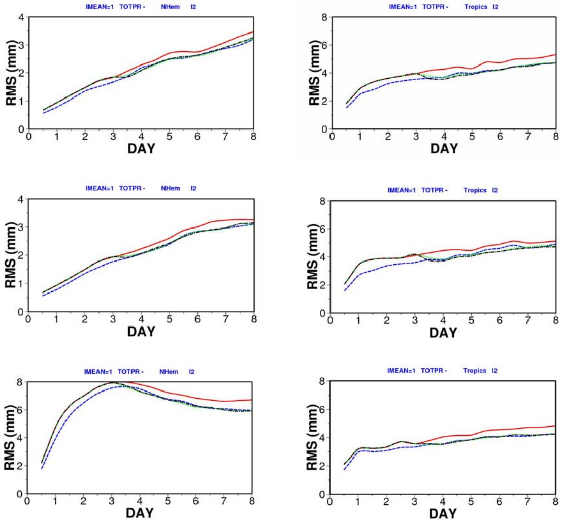
Figure 13. Top panels: average spread (STD) of 12-hour accumulated total precipitation (TP12) over NH (left) and the tropics (right) for the T399 (red solid lines), T255 (blue dashed lines), VAR3-OV-24HD (green dotted lines) and VAR3 (black chain-dashed lines) ensembles run with real orography. Middle panels: as top panels but for ensembles run with flat orography. Bottom panels: as top panels but for ensembles run in aqua-planet mode. Values are expressed in mm.
