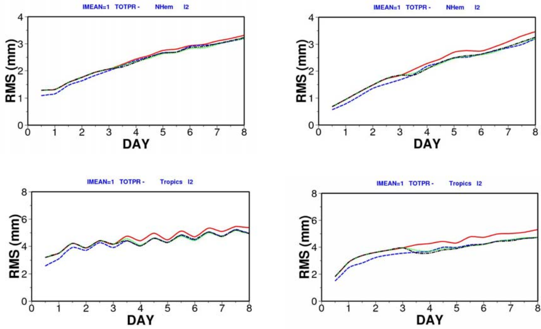
Figure 3 Top panels: average RMSE of the EPS perturbed-forecasts (left) and average spread (STD, right) of 12-hour accumulated total precipitation (TP12) over NH for the T399 (red solid lines), T255 (blue dashed lines), VAR3-OV-24HD (green dotted lines) and VAR3 (black chain-dashed lines) ensembles. Bottom panels: as top panels but for TP12 over the tropics. Values are expressed in mm.
