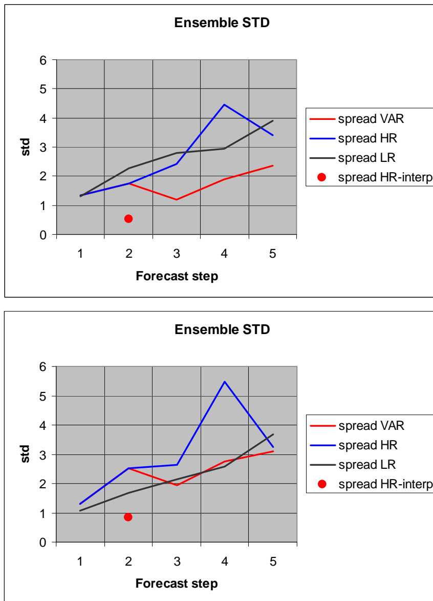
Figure 16. Spread (STD) of the high-resolution (HR, blue lines), low-resolution (LR, black-lines) and variable-resolution (VAR, red lines) idealized ensembles for two cases (see section 4 for more details). The red solid circle denotes the STD of the HR-fields after having been interpolated on the low-resolution grid.
