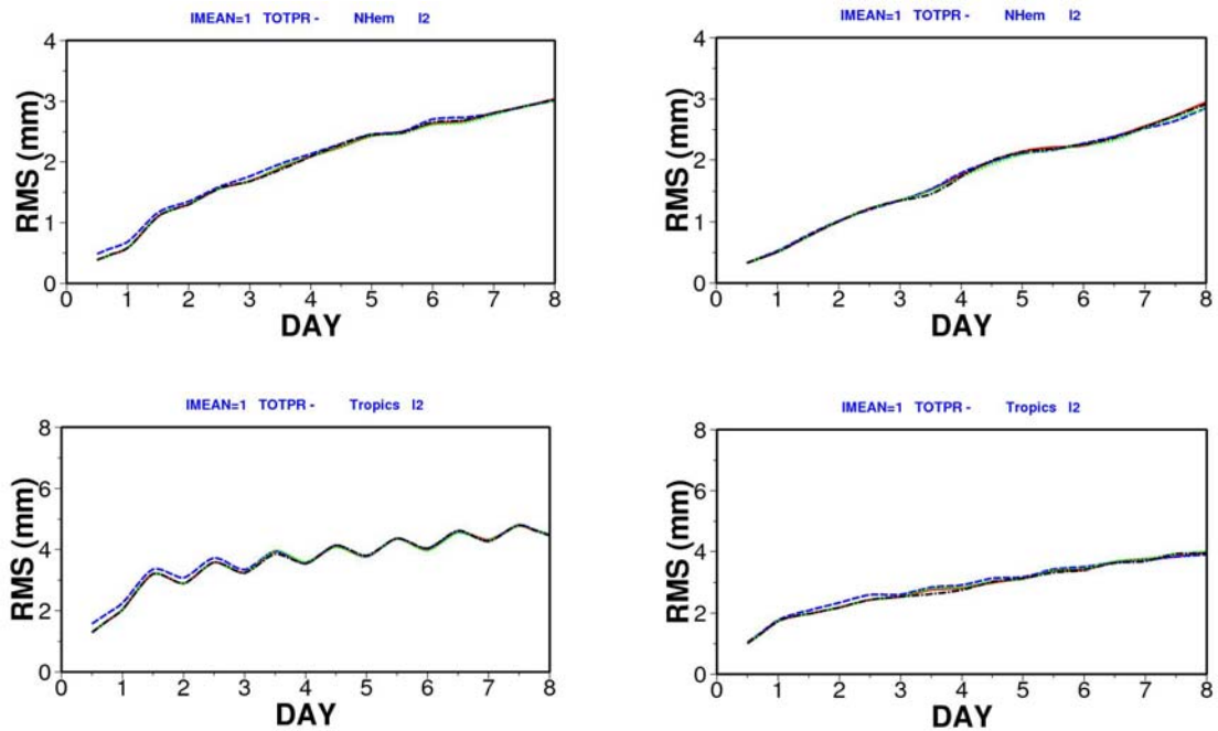
Figure 4. As Fig. 3 but for after T63 filtering. Top panels: average RMSE of the EPS perturbed-forecasts (left) and average spread (STD, right) of the T63-filtered 12-hour accumulated total precipitation (TP12) over NH for the T399 (red solid lines), T255 (blue dashed lines), VAR3-OV-24HD (green dotted lines) and VAR3 (black chain-dashed lines) ensembles. Bottom panels: as top panels but for filtered TP12 over the tropics. Values are expressed in mm.
