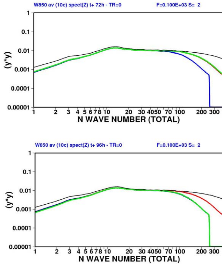
Figure 10. As Fig. 5 but for the spectra of the squared ensemble forecasts of the squared vertical velocity at 850 hPa ( W850^2 ) for the T399 (red solid lines), T255 (blue solid lines), VAR3-OV-24HD (black solid lines) and VAR3 (green solid lines) ensembles at t+72h (top panel) and at t+96h (bottom panel). The thin black solid line visible in both panels shows the spectra of the T799 ECMWF verifying analysis. At t+72h , the T399 and VAR3-OV-24HD curves coincide with the VAR3 line and thus are not visible, while at t+96h the VAR3-OV-24HD and VAR3 curves are very similar to the T255 curve. W850^2 values (in ms^{-1} ) have been multiplied by 10^{-2} .
