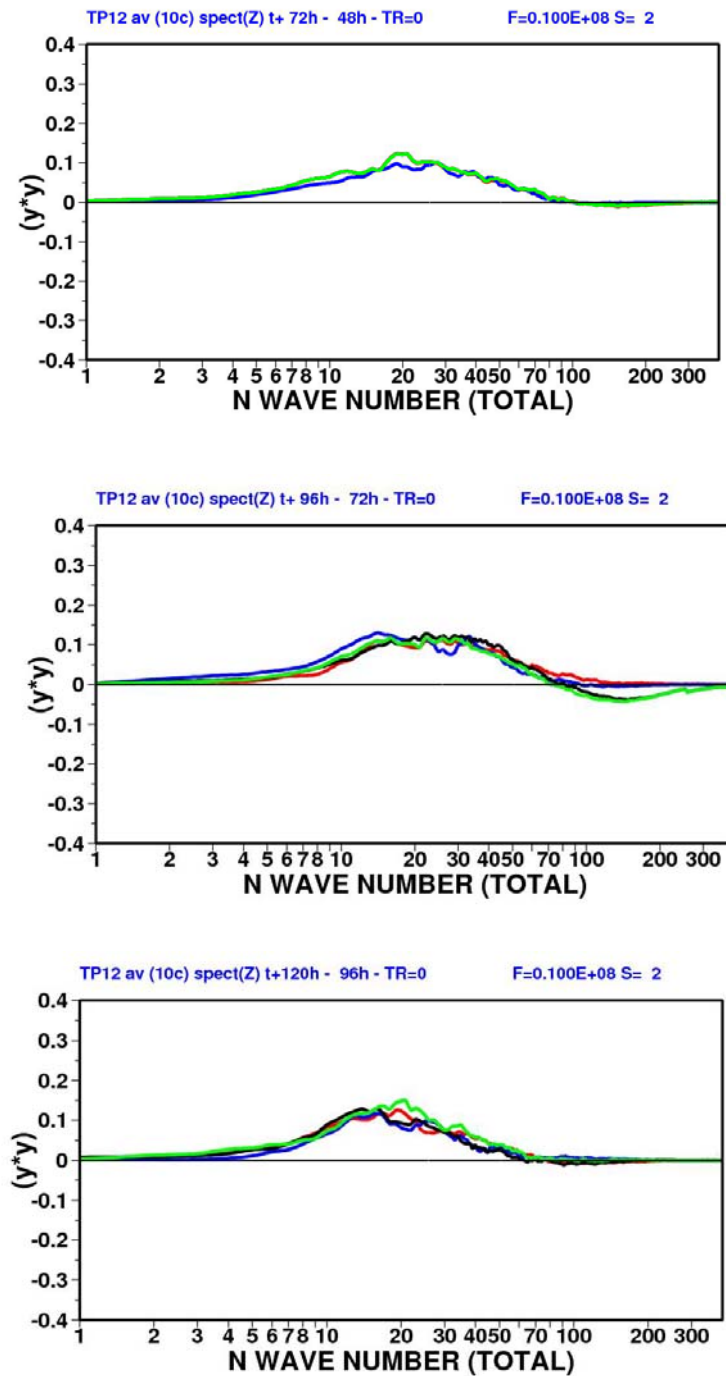
Figure 6 Difference between the variance ( STD^2 ) spectra of 12-hour accumulated total precipitation (TP12) for the T399 (red solid lines), T255 (blue solid lines), VAR3-OV-24HD (black solid lines) and VAR3 (green solid lines) ensembles: [ STD^2(72h)-STD^2(48h) ] (top panel), [ STD^2(96h)-STD^2(72h) ] (middle panel) and [ STD^2(120h)-STD^2(96h) ] (bottom panel). In the first panel, the T399 and VAR3-OV-24HD curves coincide with the VAR3 line and thus are not visible. STD^2 differences (in m^2 ) have been multiplied by 10^7 .
