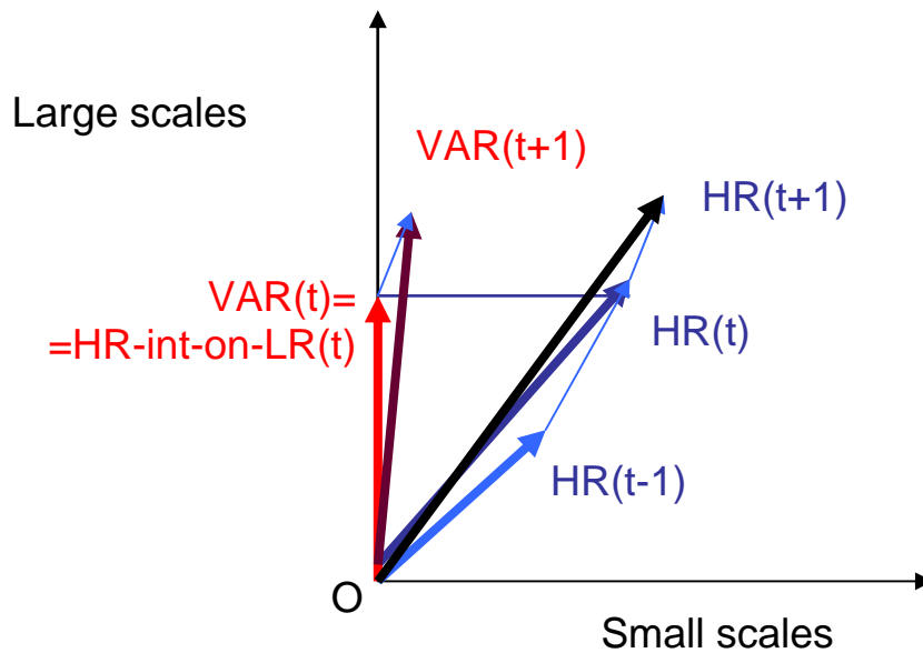
Figure 17. Schematic of the impact of the VAREPS truncation on the total precipitation spread (STD) large- and small-scale components. Vectors starting at the origin represent the ensemble spread at a specific forecast time. \|HR(t-1)\| and \|HR(t)\| are the HR-IEPS STD 1-day before and at the truncation time t , and \|HR(t)-HR(t-1)\| is the increase in STD between (t-1) and t . At time t , the VAR( t ) STD is equal to the HR( t ) STD. But the interpolation of the HR( t ) fields onto the LR-grid sets to zero the small-scale component of the VAR fields. As a result, \|VAR(t+1)\| , which is the STD of the VAR ensemble, can be smaller than \|VAR(t)\|=\|HR(t)\| , which is the STD of the VAR ensemble the day before. This results in a decrease in the STD of the VAR ensemble during the first day after the truncation time.
