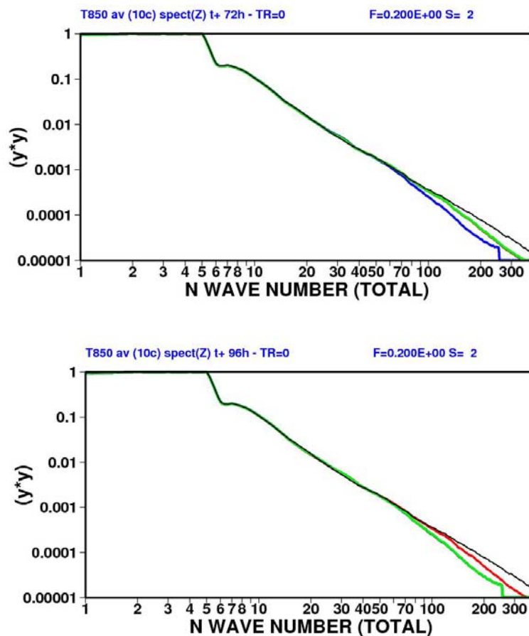
Figure 7 As Fig. 5 but for the spectra of the squared ensemble forecasts of the 850hPa temperature ( T850^2 ) for the T399 (red solid lines), T255 (blue solid lines), VAR3-OV-24HD (black solid lines) and VAR3 (green solid lines) ensembles at t+72h (top panel) and at t+96h (bottom panel). The thin black solid line visible in both panels shows the spectra of the T799 ECMWF verifying analysis. At t+72h , the T399 and VAR3-OV-24HD curves coincide with the VAR3 line and thus are not visible, while at t+96h the VAR3-OV-24HD and VAR3 curves are very similar to the T255 curve. T850^2 values (in degrees) have been multiplied by 5.
