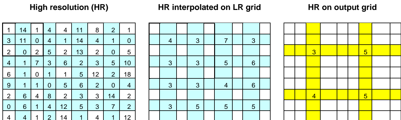
Figure 15. Example of one idealized high resolution field (left) and its interpolated field on the coarser production grid (middle) and on the coarsest output grid (right panel).
