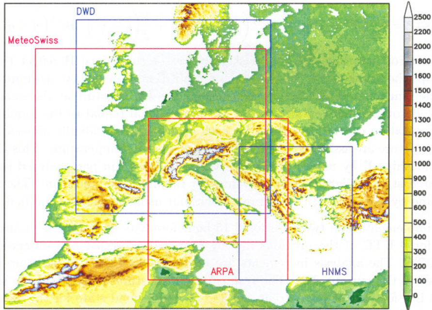
Figure 2: LM integration domains at DWD, MeteoSwiss, ARPA-SMR and HNMS
