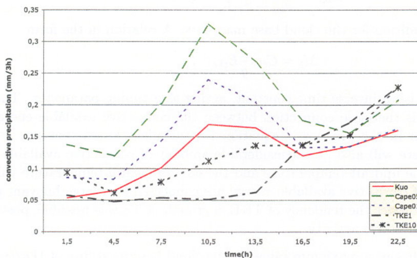
Figure 16: Left: Area-average of convective precipitation for 23 July 1998 00 UTC as function of forecast time (see text), using various variants of mass-flux closure.
