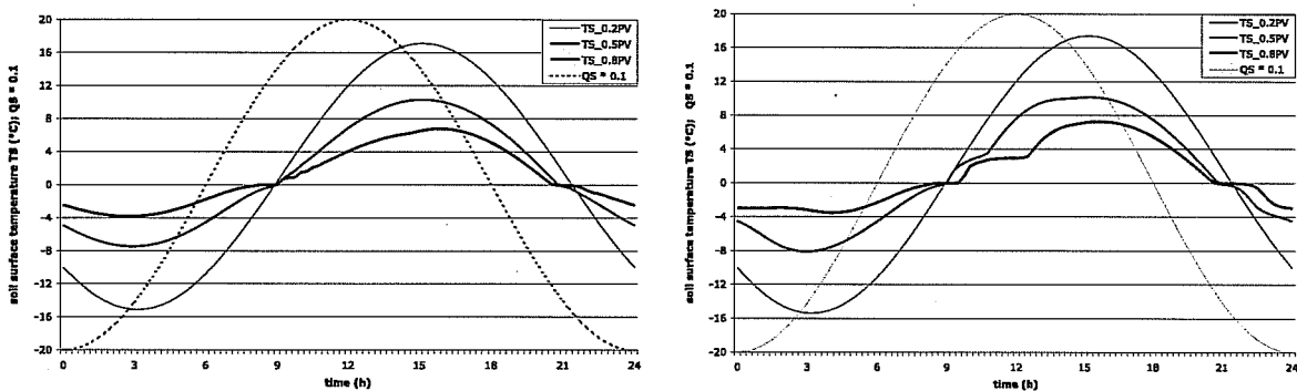
Figure 22: Soil surface temperature (°C) for a harmonic thermal forcing (dotted) and different water contents (see text). Freezing and melting at a threshold temperature depending on soil moisture and soil type. Left: 200-layer version. Right: 6-layer version.
