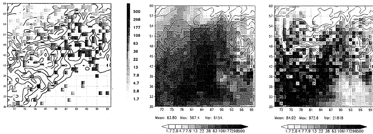
Figure 12: 24-h accumulated precipitation for the Brig case, 23 September 1993 6 UTC – 24 September 1993 6 UTC. Left: Observations; middle: LM-simulation using the prognostic precipitation scheme; right: LM-simulation using the operational precipitation scheme. The (x,y) gridpoint indices of Brig are (83,48).
