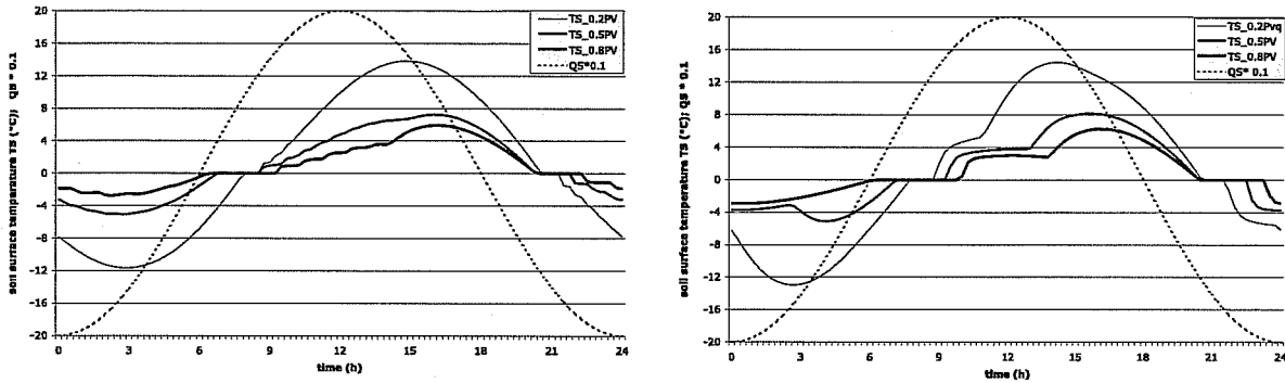
Figure 21: Soil surface temperature (°C) for a harmonic thermal forcing (dotted) and different water contents (see text). Freezing and melting at freezing point. Left: 200-layer version. Right: 6-layer version.
