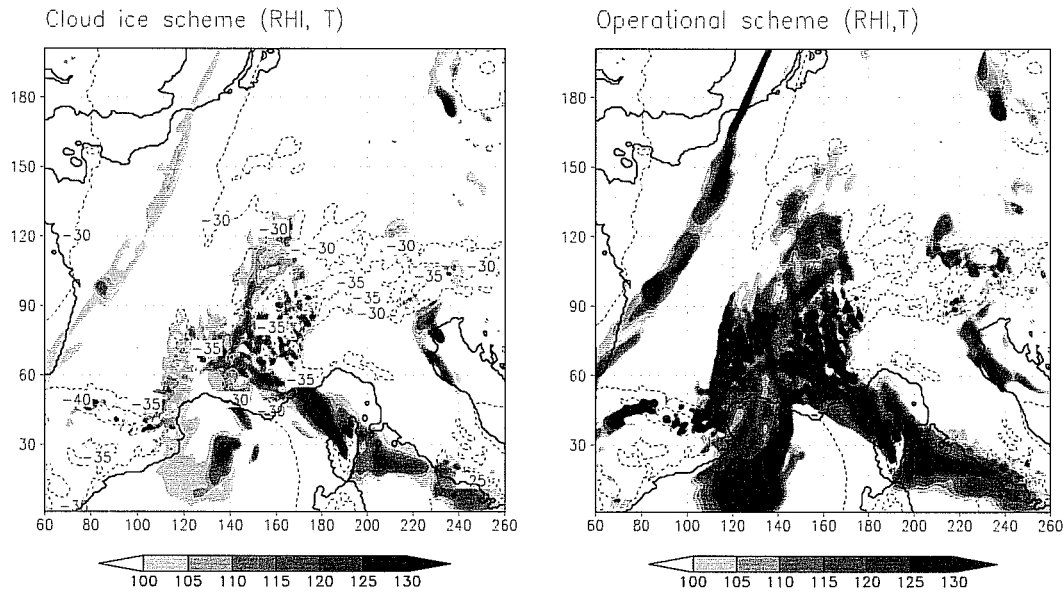
Figure 10: Relative humidity over ice (shaded, in %) and temperature ( ^{\circ}\text{C} , isolines) for 4 May 2001 00 UTC + 12 h at model level 14. Left: cloud ice scheme. Right: operational scheme.
