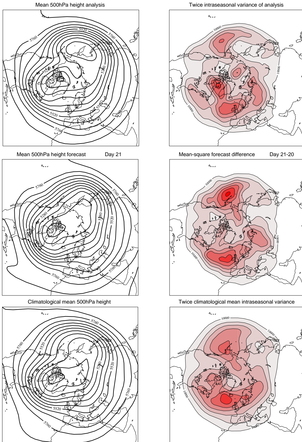
Fig 12. Mean 500hPa height fields (left, contour interval 80m) from analyses for the period from 12 December 2000 to 11 March 2001 (upper), from 21-day T255L40 forecasts verifying in the period (middle) and from a corresponding 22-year climatology (lower). The plots on the right show (contour interval 10000m 2 ) twice the intraseasonal variance of analyses for the period (upper), the mean-square differences between 21-day and 20-day forecasts verifying in the period (middle) and twice the corresponding mean intraseasonal variance from the 22-year climatology (lower).
