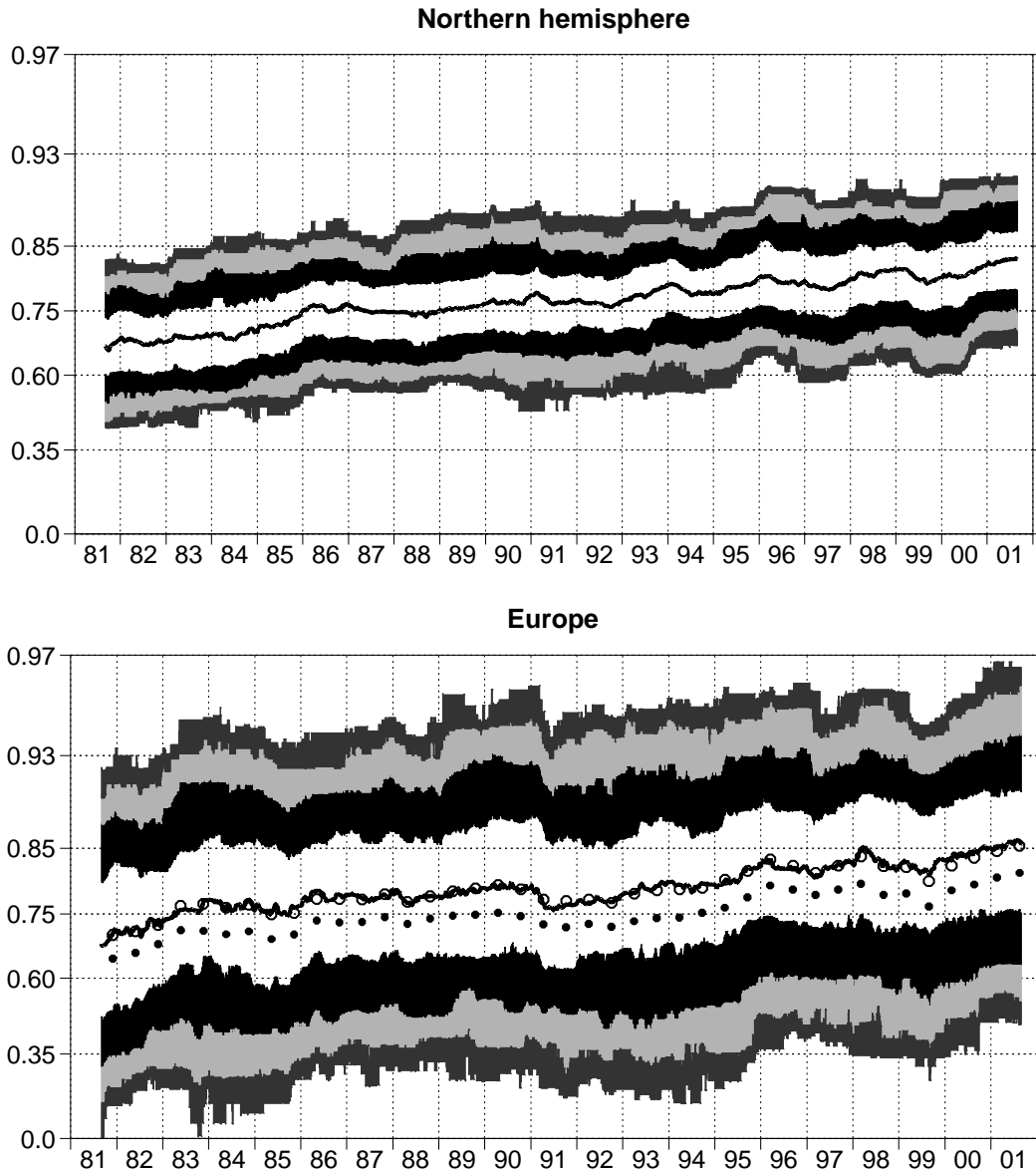
Fig 5. Time series of day-5 500hPa height anomaly correlation coefficients based on operational ECMWF forecasts with initial dates from 27 July 1980 to 31 August 2001 for the northern hemisphere (upper) and Europe (lower). The black lines show the median of running 401-day sequences of daily correlations. The shaded bands indicate the ranges of correlations which lie between the 2nd and 4th, the 4th and 10th, and the 10th and 25th percentiles of the 401-day distributions, and also between the 75th and 90th, the 90th and 96th, and the 96th and 98th percentiles. The ordinates are linear in the Fisher transform of the anomaly correlations. The black dots and open circles plotted for Europe denote the running means discussed in the text. Values plotted for a particular day relate to the 401-day period ending on that day.
