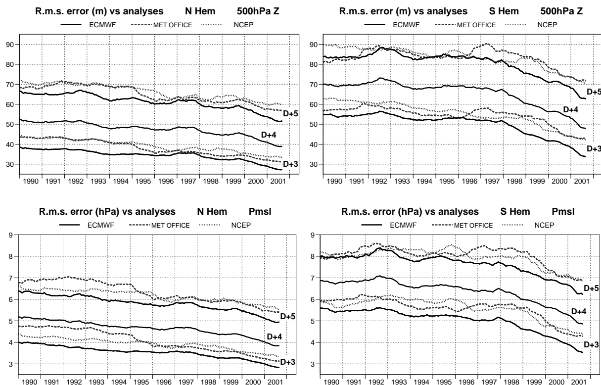
Fig 1. Root-mean-square errors of 3- and 5-day forecasts of 500hPa height (upper; m) and mean-sea-level pressure (lower; hPa) for the extratropical northern (left) and southern (right) hemispheres. Results from ECMWF, the Met Office and NCEP are plotted in the form of annual running means of all monthly data exchanged by the centres from January 1989 to August 2001. ECMWF 4-day forecast errors are also shown. Values plotted for a particular month are averages over that month and the 11 preceding months, so that the effect of a forecasting-system change introduced in that month is seen from then onwards.
