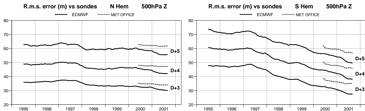
Fig 3. Root-mean-square errors of 3-, 4- and 5-day ECMWF 500hPa height (m) forecasts for the extratropical northern (left) and southern (right) hemispheres, plotted in the form of annual running means of monthly data for verification against radiosondes from July 1994 to August 2001. Recent Met Office forecast errors are also shown. Values plotted for a particular month are averages over that month and the 11 preceding months.
