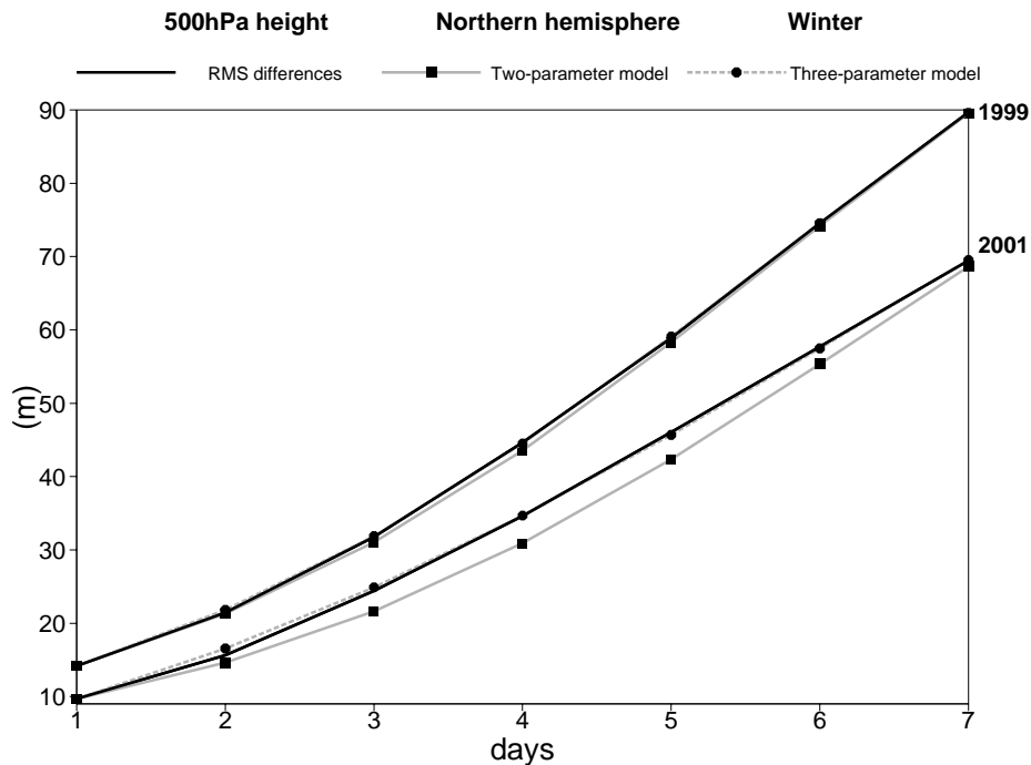
Fig 9. Root-mean-square differences between successive 500hPa height forecasts verifying at the same time (“perfect-model” errors) as functions of the forecast range, for the northern hemisphere winters of 1999 and 2001. The solid black lines denote the actual differences, the solid grey lines with square marker symbols denote the results of fitting the two-parameter error-growth model to these differences and the grey dashed curves with circular marker symbols denote the results of fitting the three-parameter model. Results are shown only to day seven so that the closeness of fit can be more easily seen.
