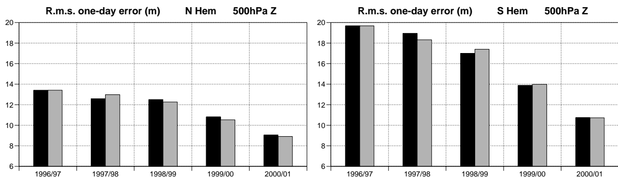
Fig 2. Root-mean-square errors of ECMWF's one-day forecasts of 500hPa height (m) for the extratropical northern (left) and southern (right) hemispheres. Twelve-month averages from September to August are plotted for the five years up to August 2001. The black bars denote the actual annual-mean errors, and the grey bars denote the errors that would have occurred had these operational forecasts been improved by exactly the average amounts as measured in the pre-operational trials of the forecasting-system changes introduced between November 1997 and November 2000.
