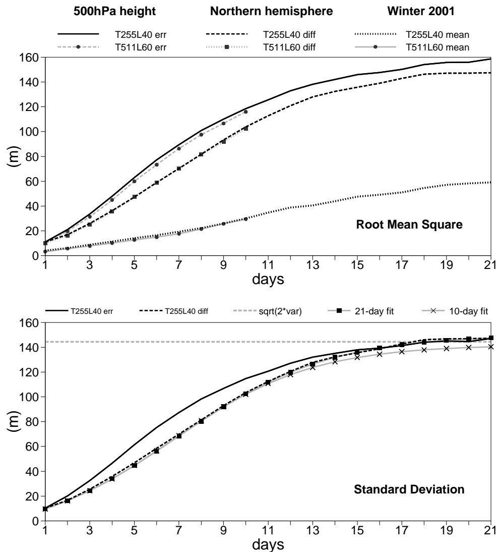
Fig 11. Root-mean-square (upper) and standard deviation (lower) of T255L40 forecast errors (solid, black) and differences between successive forecasts (dashed, black) for the forecast range up to 21 days, for northern hemisphere forecasts verifying in the period 12 December 2000 to 11 March 2001. The upper panel also shows errors and differences (grey, dashed and dotted) for corresponding T511L60 forecasts to ten days, and the root-mean-square for the hemisphere of the sample-mean T255L40 (black, dotted) and T511L60 (grey, solid) forecast errors. The lower panel includes the curves (solid, grey) that result from fitting the three-parameter error-growth model to the differences over 21 days (square marker symbols) and 10 days (crosses) and the asymptotic limit derived from the variance of analyses (dashed, grey).
