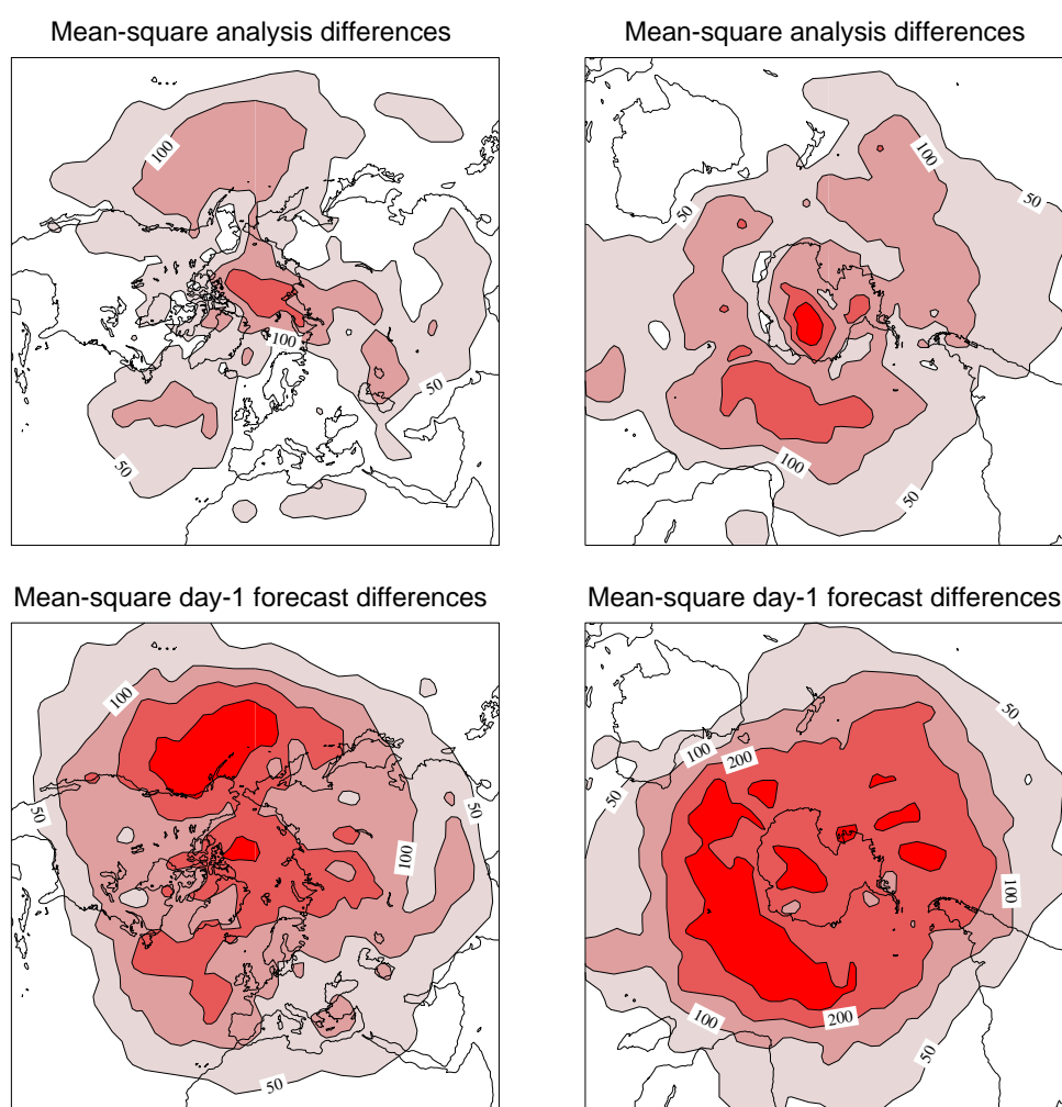
Fig 13. Mean-square differences between ECMWF and Met Office 12UTC 500hPa height analyses (upper) and one-day forecasts (lower) over the northern hemisphere (left) and the southern hemisphere (right) for the period 12 December 2000 to 11 March 2001. Contour values are 50, 100, 200 and 400\text{m}^2 . Seasonal mean differences have been excluded and smoothing has been applied to the 2.5^\circ data to reduce the amplitude of small-scale features.
