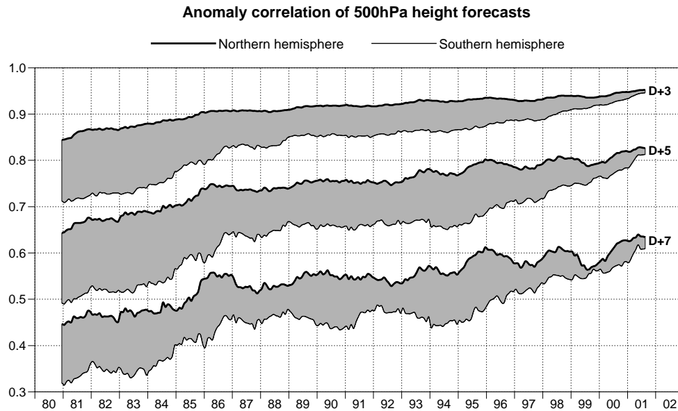
Fig 4. Anomaly correlation coefficients of 3-, 5- and 7-day ECMWF 500hPa height forecasts for the extratropical northern and southern hemispheres, plotted in the form of annual running means of archived monthly-mean scores for the period from January 1980 to August 2001. Values plotted for a particular month are averages over that month and the 11 preceding months. The shading shows the differences in scores between the two hemispheres at the forecast ranges indicated.
