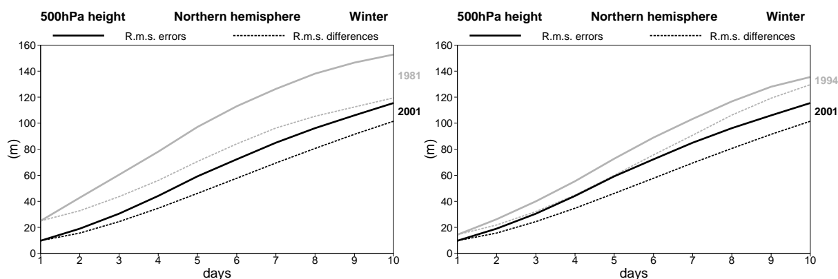
Fig 6. Root-mean-square 500hPa height forecast errors (solid) and differences between successive forecasts verifying at the same time (dashed) as functions of the forecast range, computed over the extratropical northern hemisphere, and shown for the winters of 1981 (grey) and 2001 (black) in the left panel, and for the winters of 1994 (grey) and 2001 (black) in the right panel.
