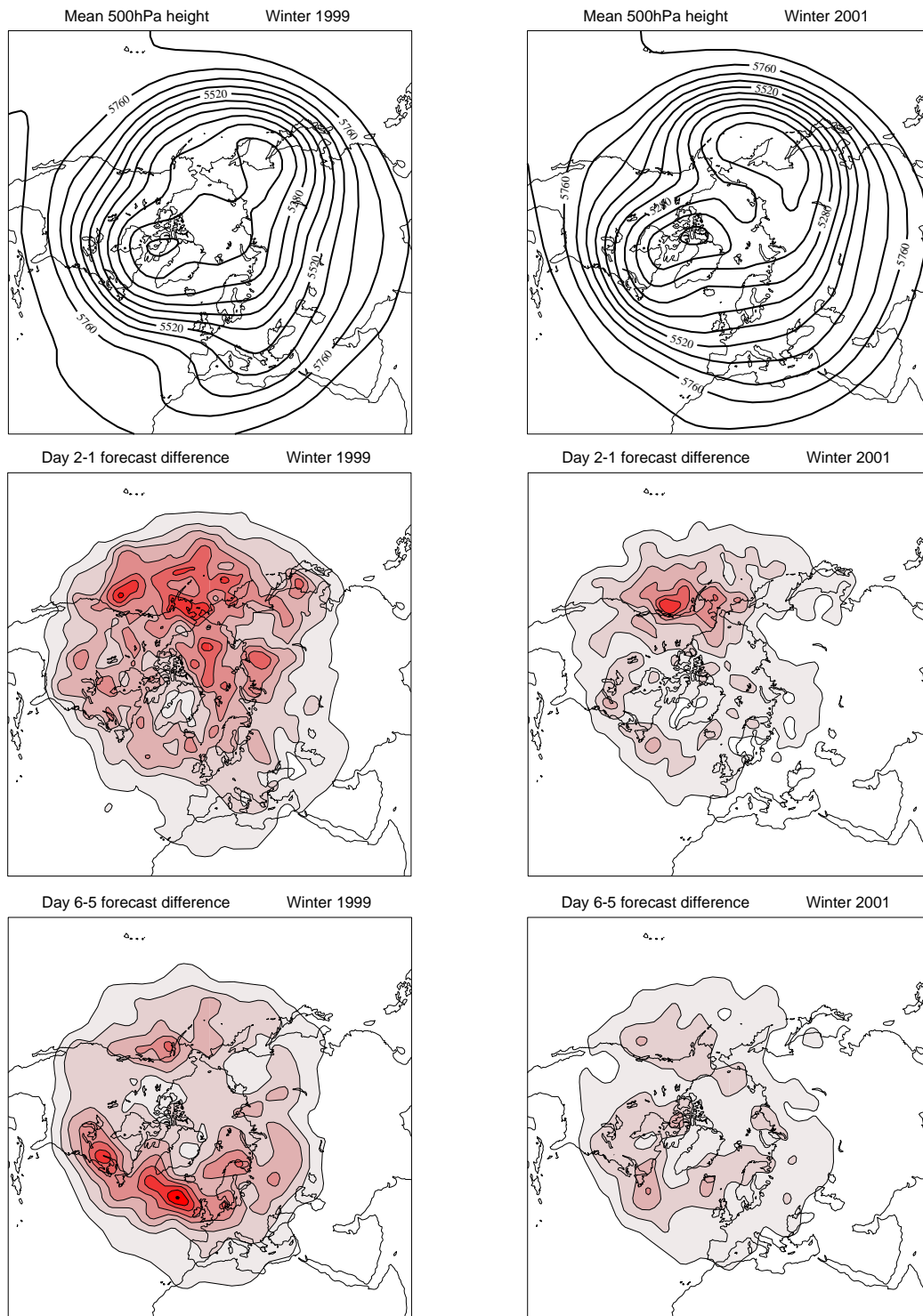
Fig 7. Mean 500hPa height fields (upper, contour interval 80m) and mean-square differences between day-2 and day-1 forecasts (middle, contour interval 200\text{m}^2 ) and between day-6 and day-5 forecasts (lower, contour interval 3000\text{m}^2 ) for the winters of 1999 (left) and 2001 (right).
