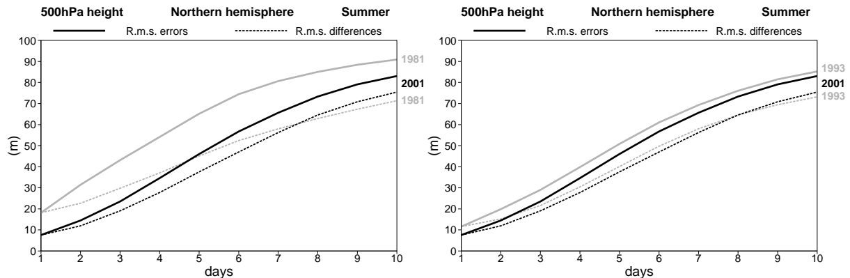
Fig 8. Root-mean-square 500hPa height forecast errors (solid) and differences between successive forecasts verifying at the same time (dashed) as functions of the forecast range, computed over the extratropical northern hemisphere, and shown for the summers of 1981 (grey) and 2001 (black) in the left panel, and for the summers of 1993 (grey) and 2001 (black) in the right panel.
