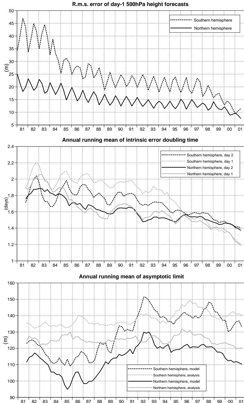
Fig 10. Root-mean-square errors of one-day 500hPa height forecasts for the extratropical northern (solid) and southern (dashed) hemispheres plotted for each season since 1981 (upper), and corresponding running annual means of the error doubling times (middle) at days one (grey) and two (black) and the asymptotic limits (lower, black) from the three-parameter error-growth model. The asymptotic limits given by the root-mean-square over the hemispheres of twice the intraseasonal variance of analyses are also shown in the lower panel (grey).
