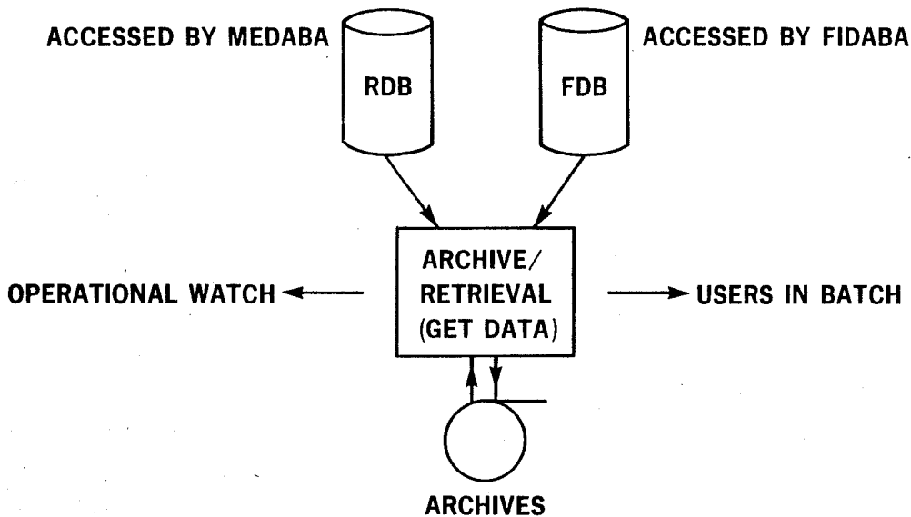
Fig. 6 The "GETDATA" Archive/Retrieval
