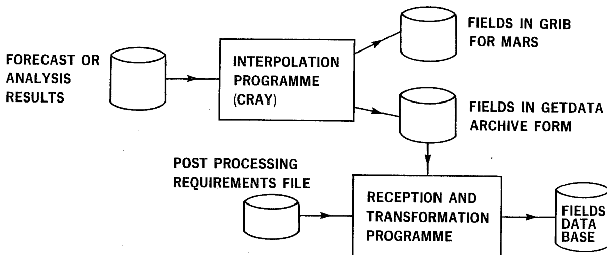
Fig. 12 Post-processing - Current status
