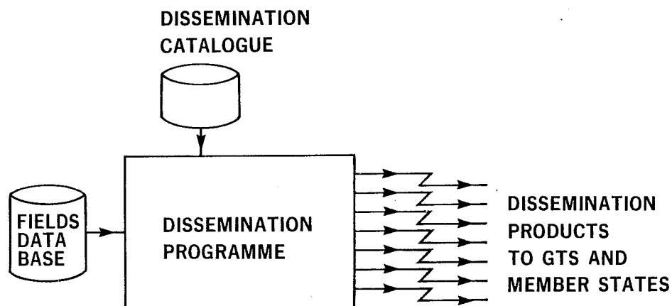
Fig. 13 Dissemination - current status
