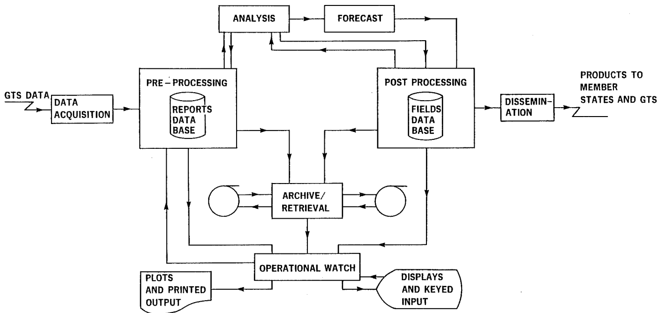
Fig. 2 ECMWF Meteorological Data Flow
